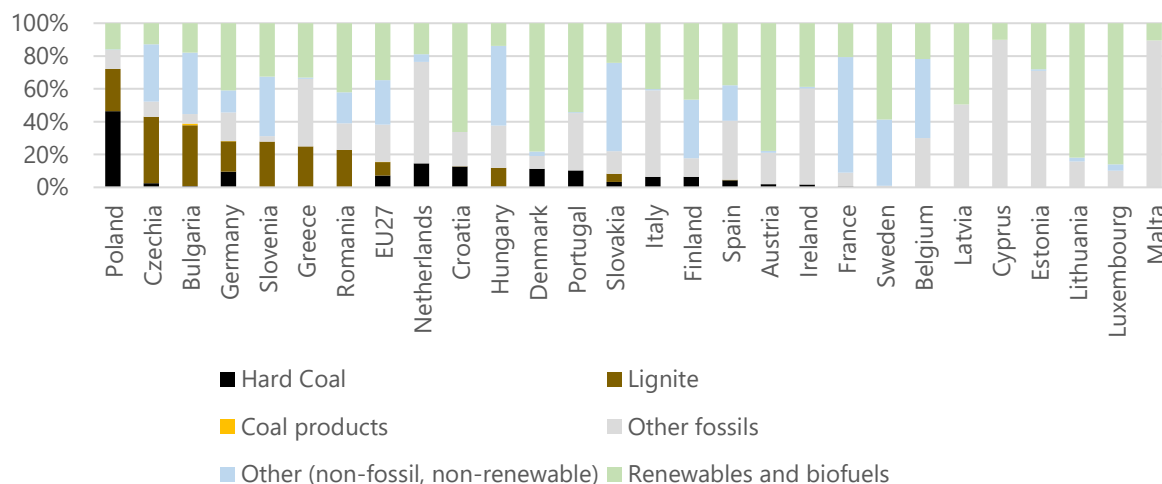
Figure 3-4: Share of coal (hard coal and lignite) in domestic gross electricity production in 2019 (in %)
