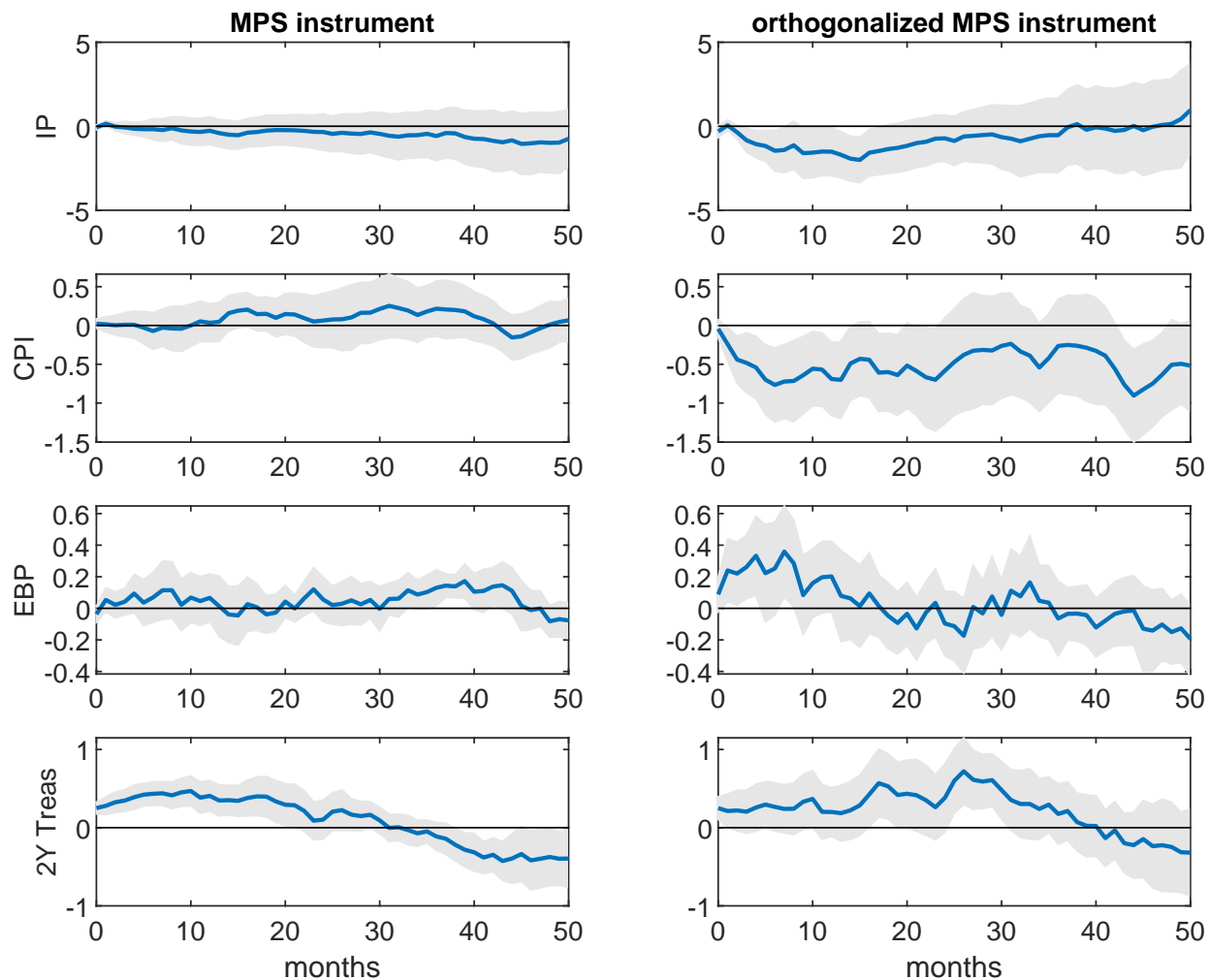
Figure 5: Local Projections
