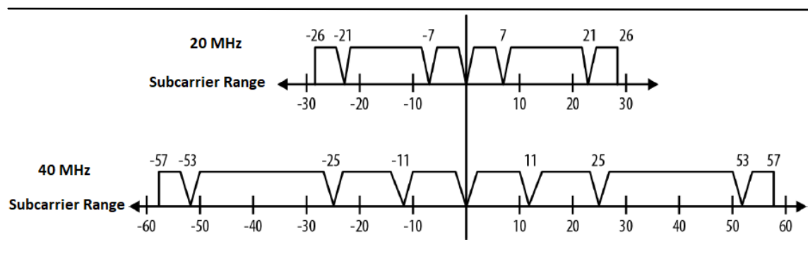
Figure B 2: Comparison between 20 MHz and 40 MHz channels in WiFi 4
