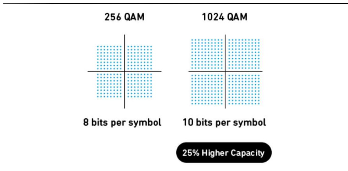
Figure B 11: Constellation maps of 256-QAM and 1024-QAM
