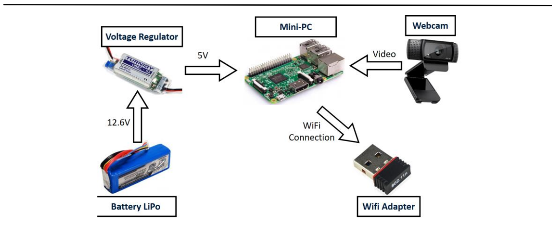
Figure C 9: WiFi in smart traffic light setting
