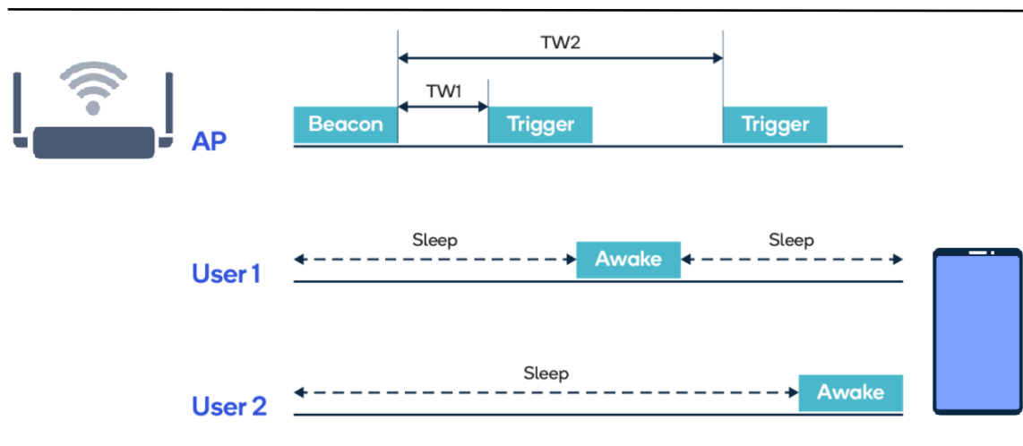
Figure B 13: TWT operation between an AP and 2 STAs
