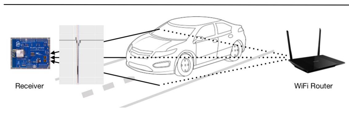
Figure C 7: Deployment plan for traffic data collecting system
