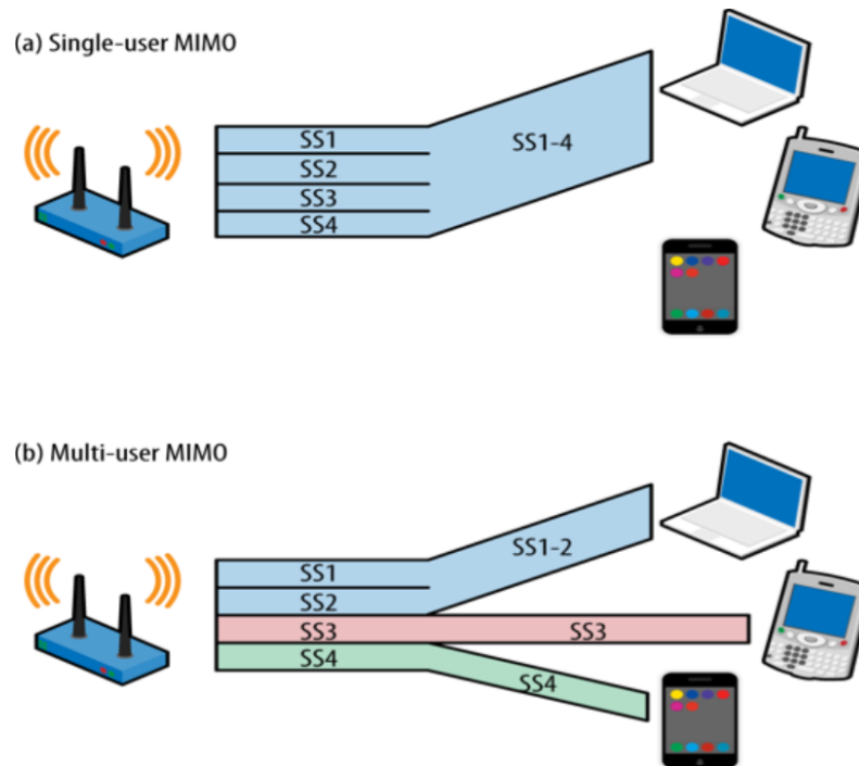
Figure B 4: Single-user MIMO vs. Multi-user MIMO
