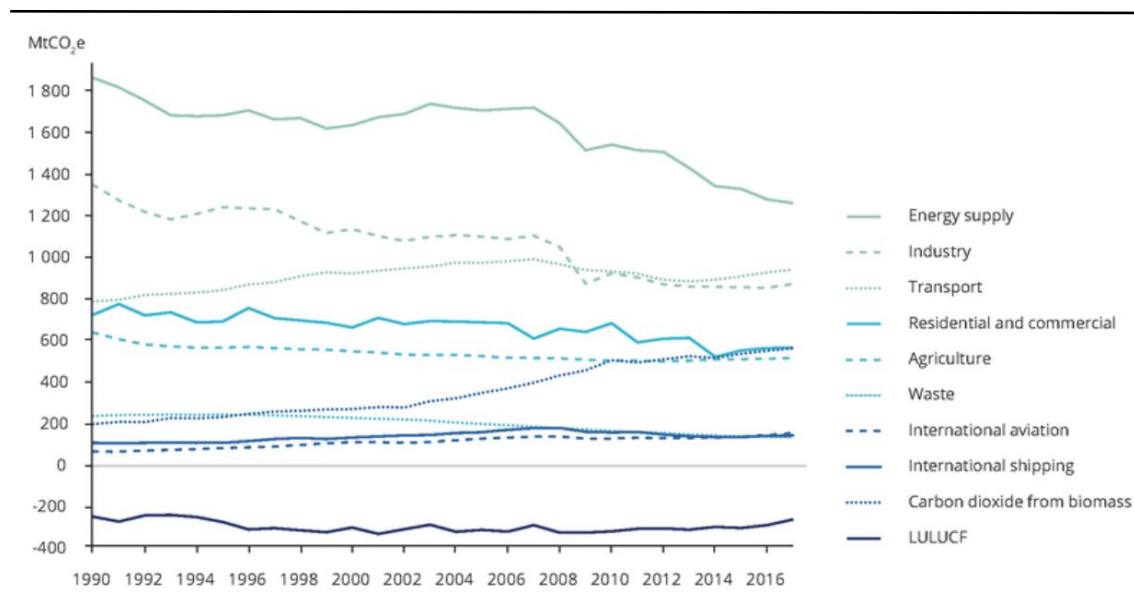
Figure 13: GHG emissions by main sector in the EU-28, 1990-2017
