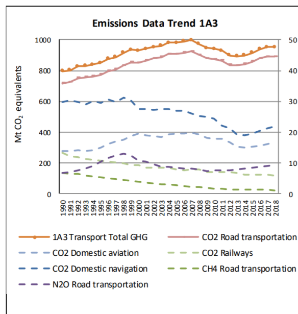
Figure 14: GHG emissions from transport in the EU
