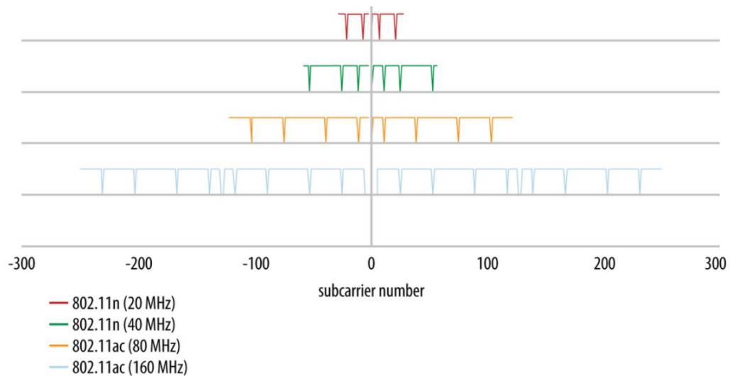
Figure B 6: WiFi 4 Channels Vs. WiFi 5 Channels
