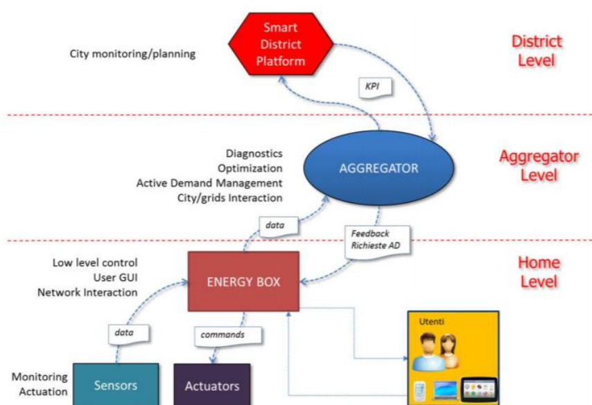
Figure C 5: Connection architecture of the Centocelle project
