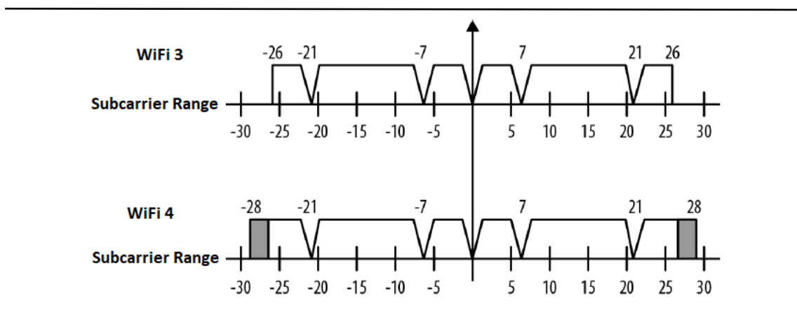
Figure B 1: Channel structure comparison between WiFi 3 (52 carriers) and WiFi 4 (56 carriers)
