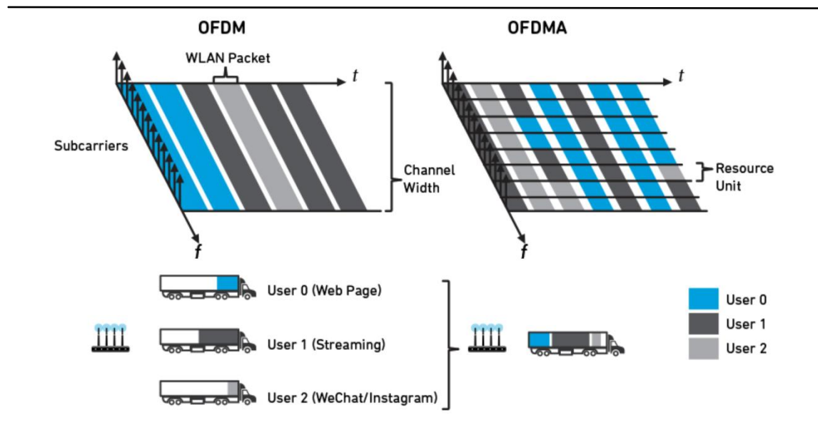
Figure B 9: OFDM Vs. OFDMA
