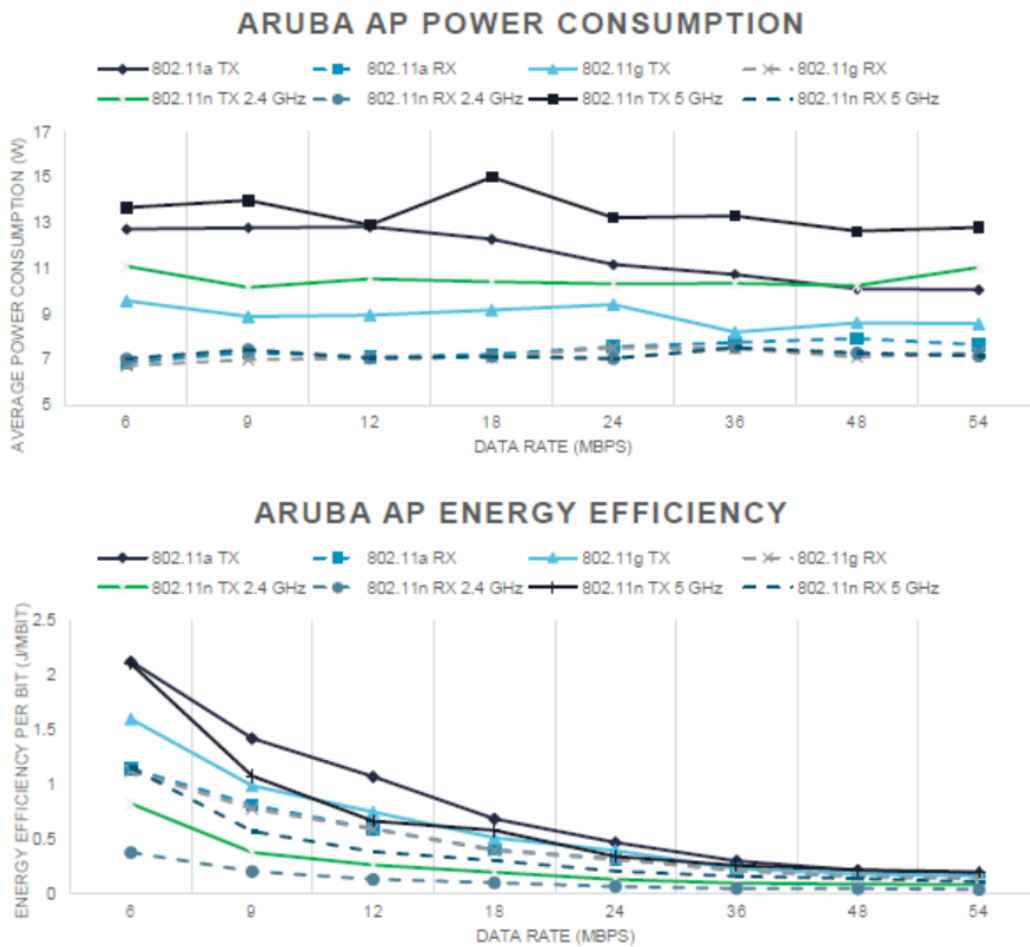
Figure 8: Power consumption and energy efficiency per Mbit of the Aruba AP
