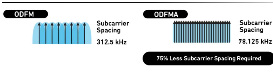
Figure B 10: Subcarrier spacing change in WiFi 6
