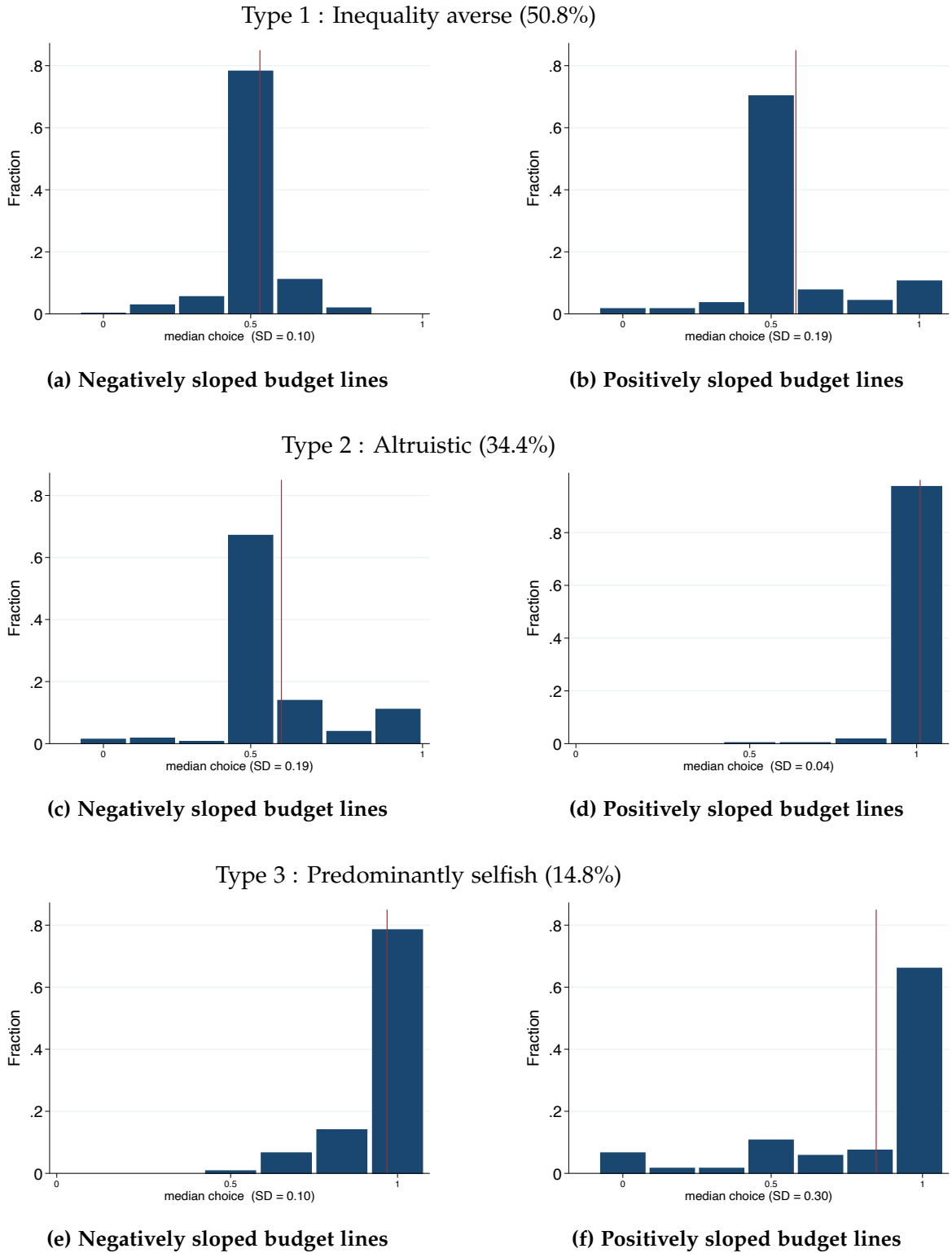
Figure 4: Distribution of individuals' median choices for each preference type.
