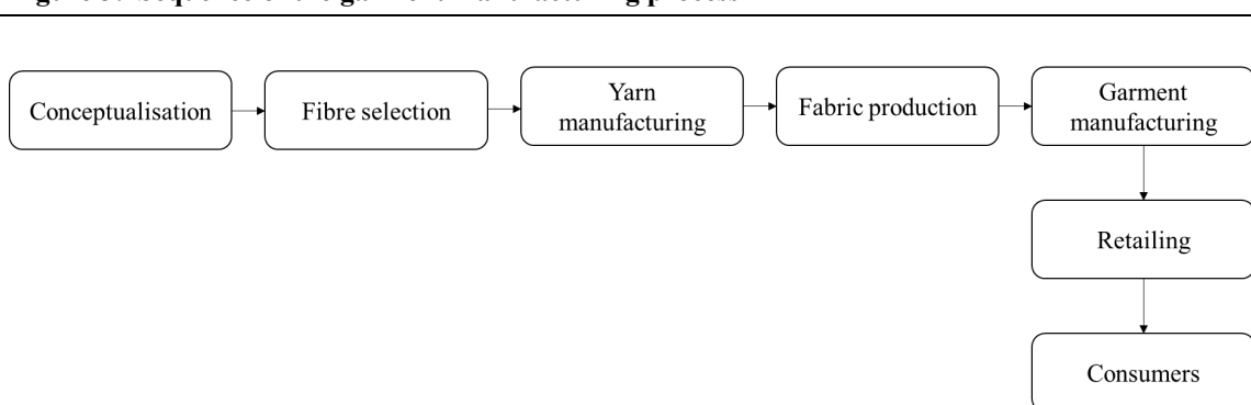
Figure 3: Sequence of the garment manufacturing process
