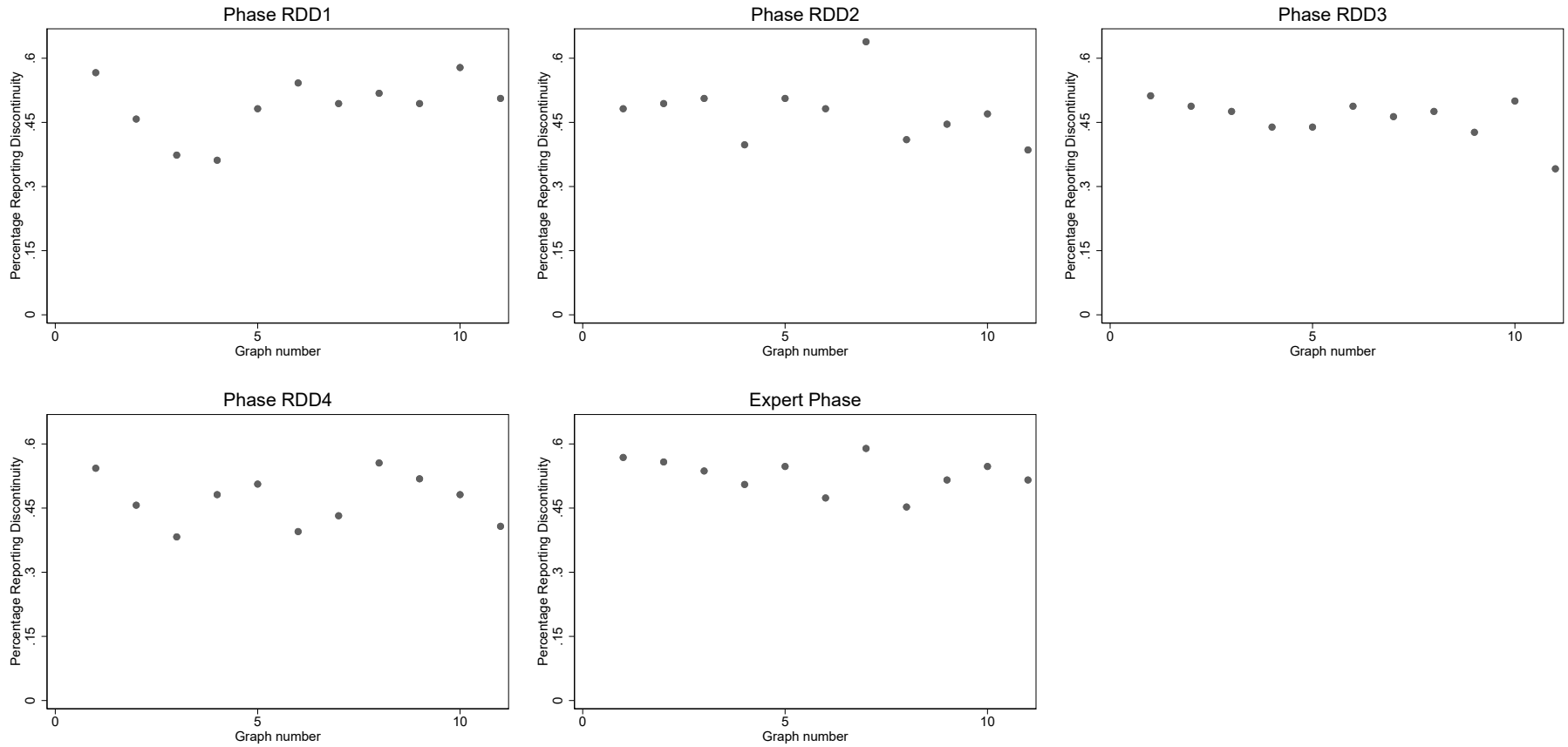
Figure A.26: Discontinuity Classifications over 11 Graphs
