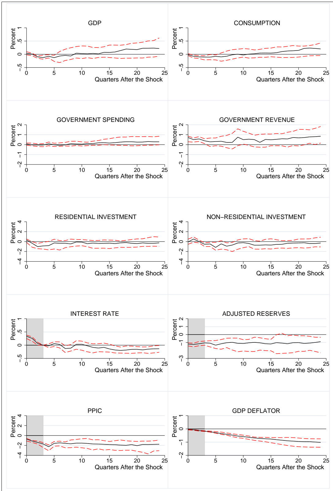
Figure 2: The monetary policy shock ordered second. The shaded areas indicate the impulses directly restricted by the identification procedure.
