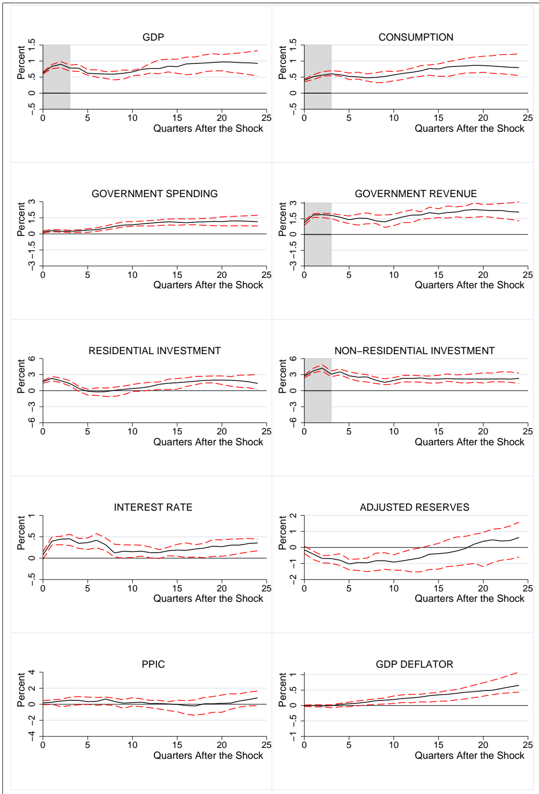
Figure 1: The business cycle shock ordered first. The shaded areas indicate the impulses directly restricted by the identification procedure.
