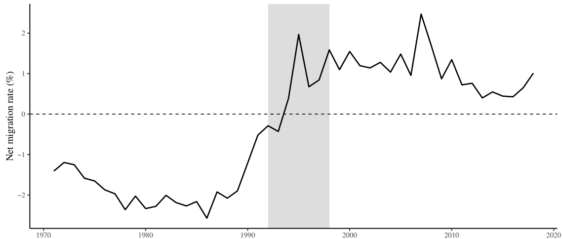
Figure 3: Net migration rate in North Bohemian municipalities (1971–2015)
