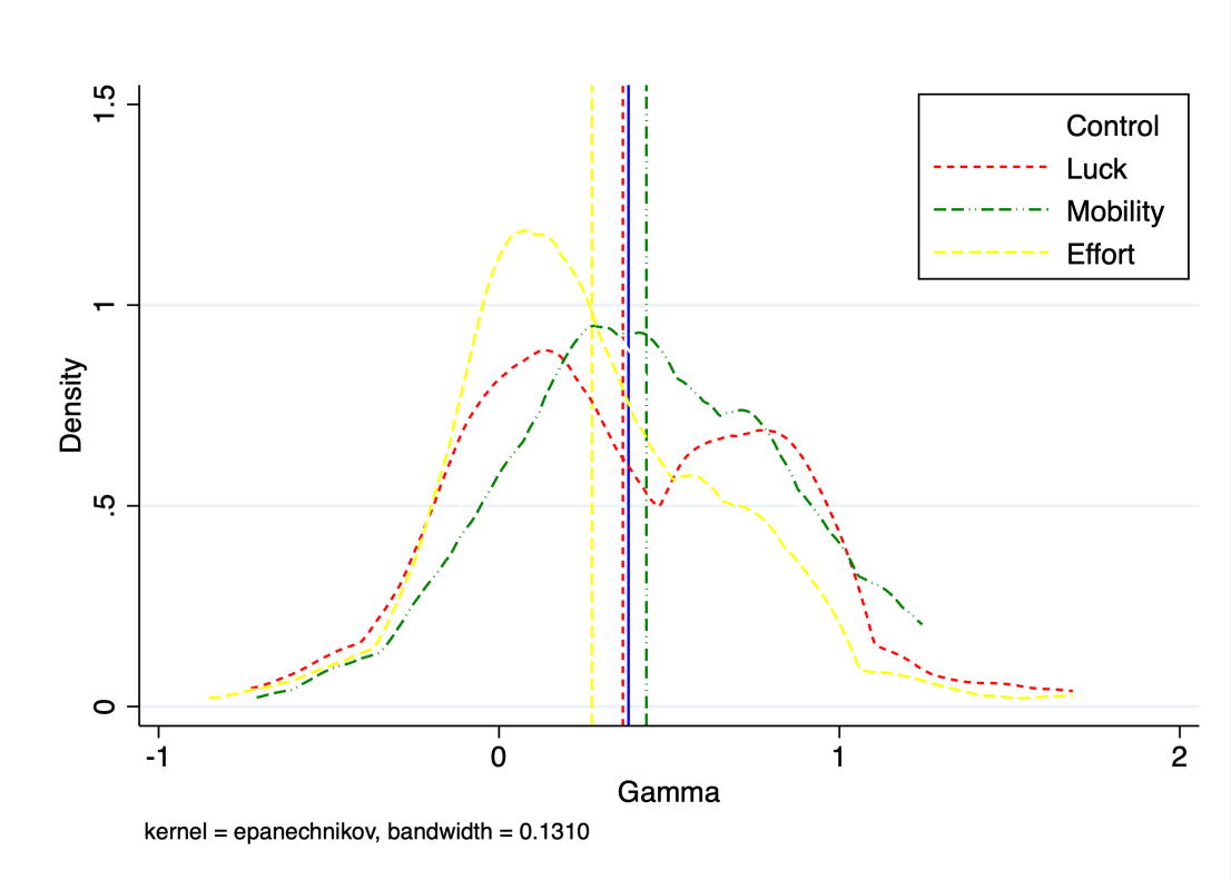
Figure A.10.1: Kernel density estimation. Treatment effect for non self-centered inequality aversion
