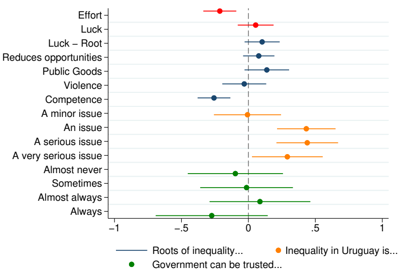
Figure A.11.2: Interpreting Gamma - Intervals regression. Estimates based on fairness treatment at individual level
