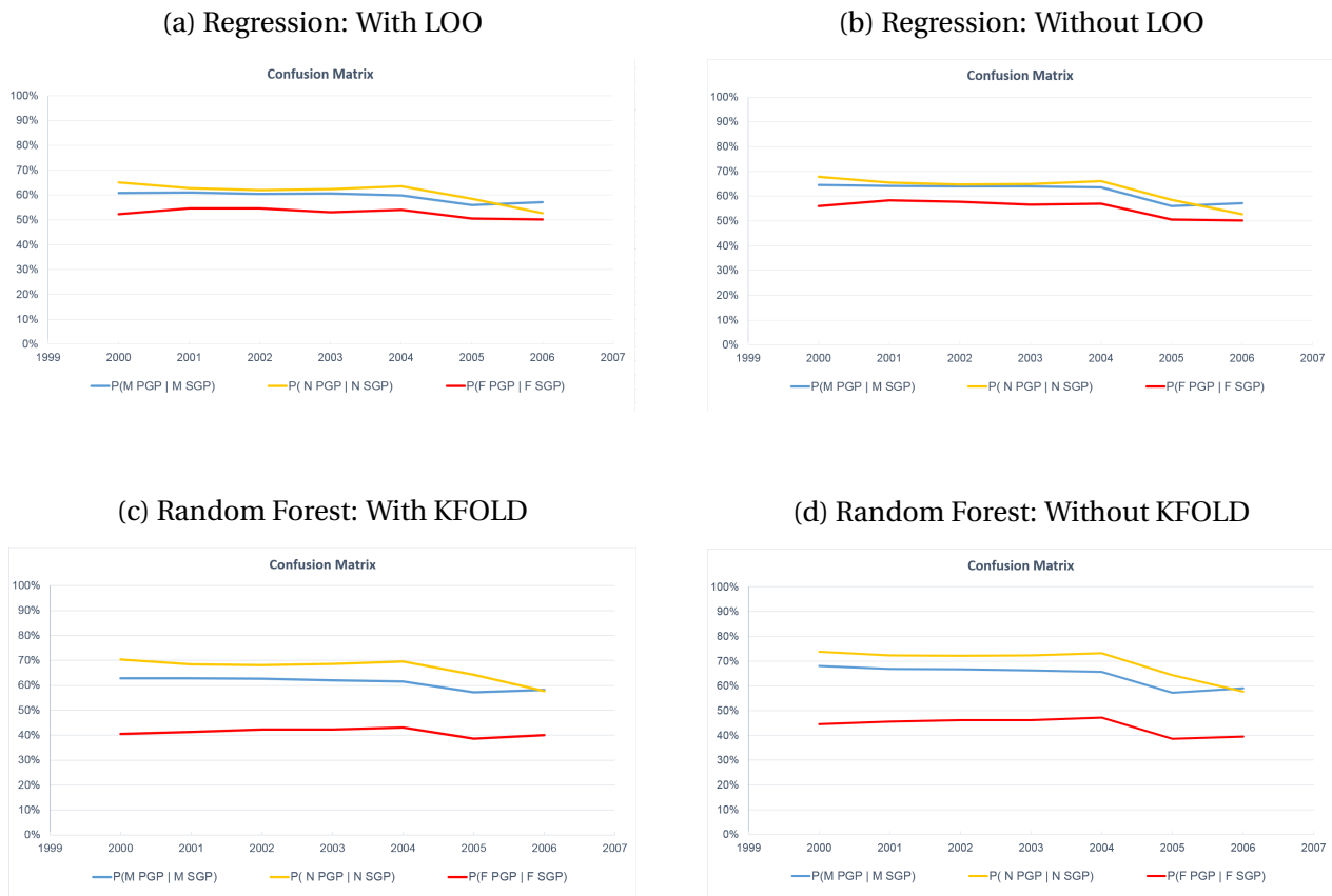
Figure C.1: Prediction Quality
