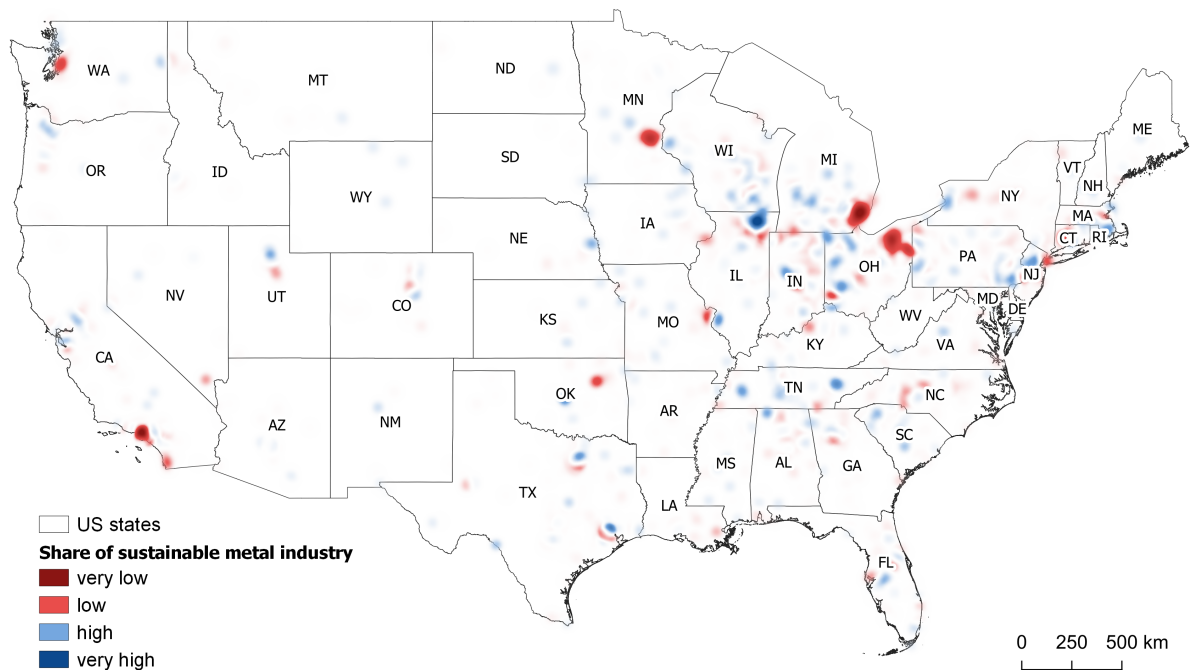
Figure 1: Heat map of the distribution of sustainable metal industry companies. The map was based on the combination of two separate bi-square kernel density maps with a pixel size of 1 km: one based on the locations of the sustainable and one for the non-sustainable metal industry. These were then normalised and subtracted from each other, creating a new raster with positive values in areas with a high (normalised) count of sustainable company locations.
