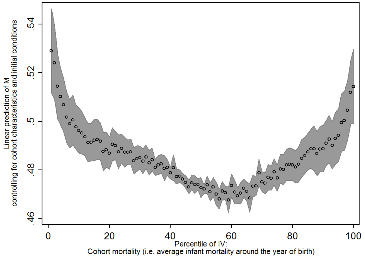
Figure 9: Cohort mortality and intergenerational persistence \beta
