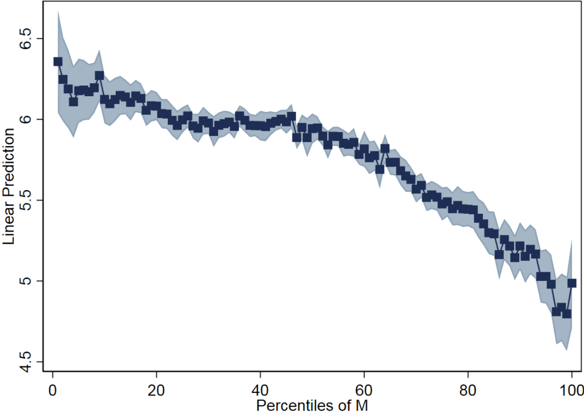
Figure 8: Non-linear relationship between social mobility and development. Intergenerational persistence \beta
