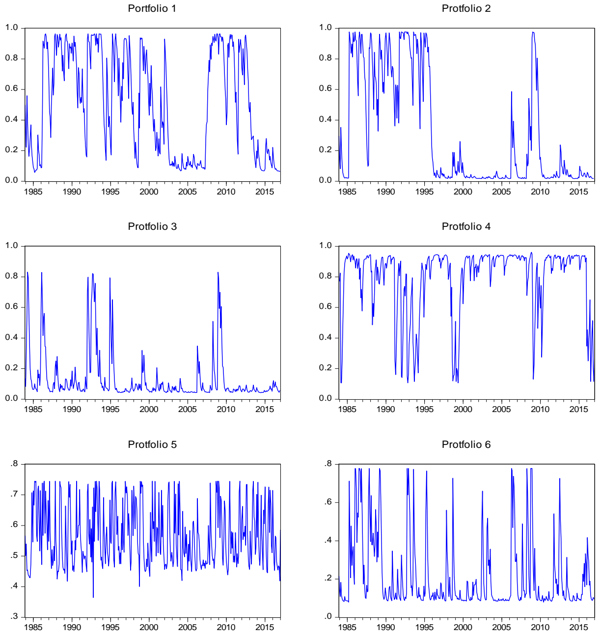
Figure 3: Regime probabilities
