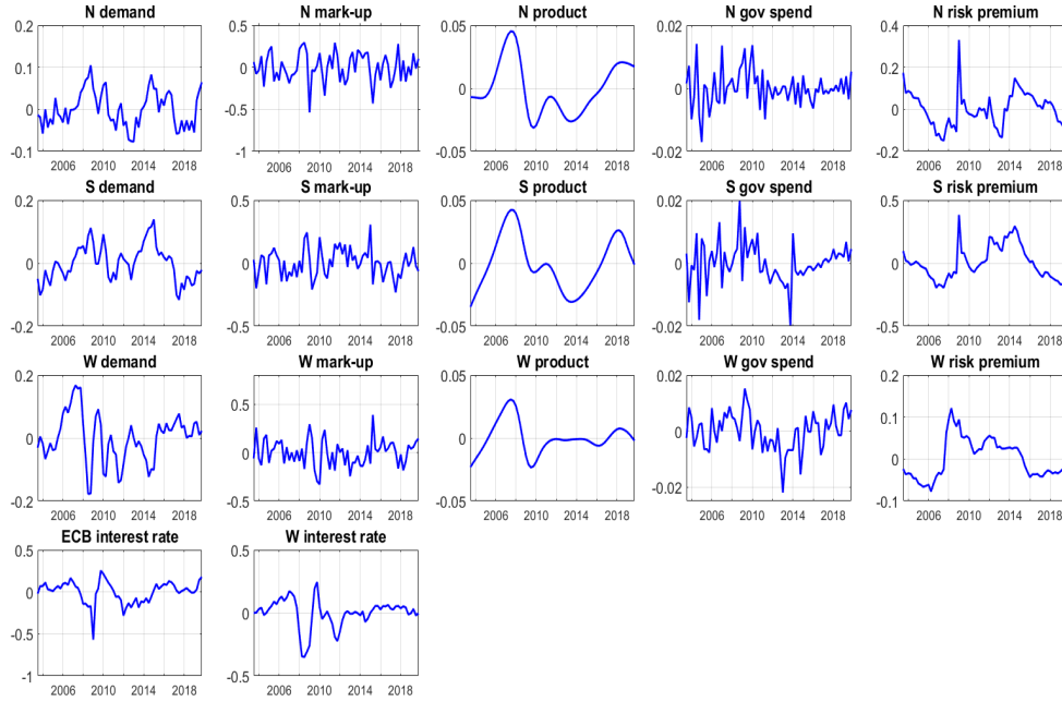
Figure 5: Historical shocks
