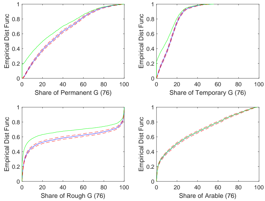
Figure 16: Kaplan-Meier estimates for 1976 with 95% confidence bounds. Estimates ignoring the censoring problem are presented in green colour.
