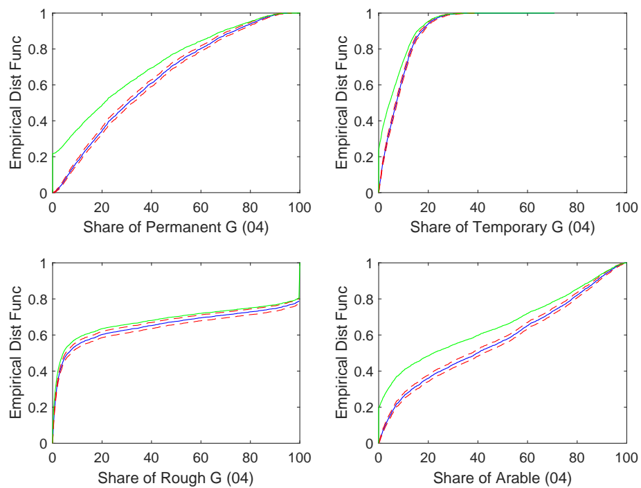
Figure 18: Kaplan-Meier estimates for 2004 with 95% confidence bounds. Estimates ignoring the censoring problem are presented in green colour.
