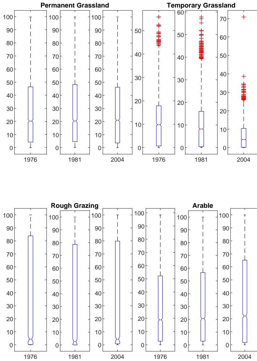
Figure 1: Boxplots
