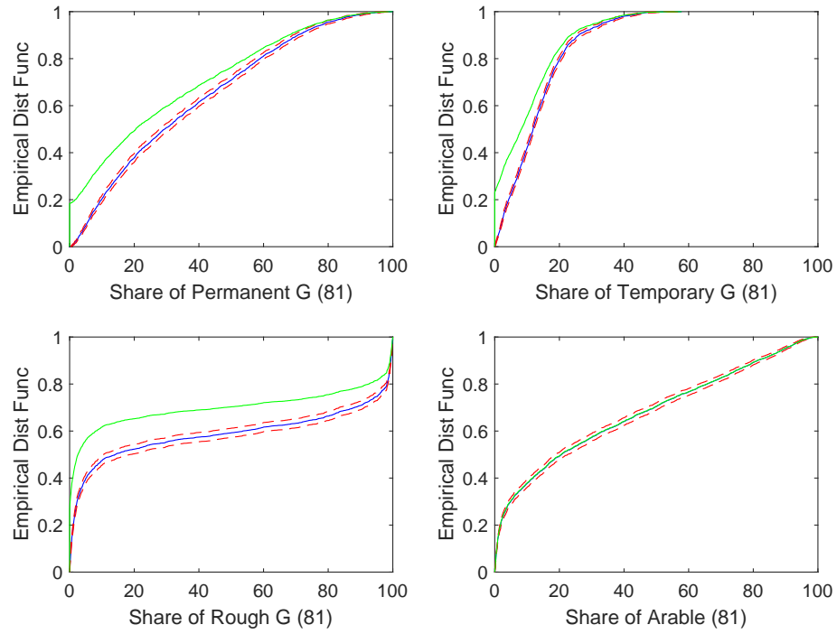
Figure 17: Kaplan-Meier estimates for 1981 with 95% confidence bounds. Estimates ignoring the censoring problem are presented in green colour.
