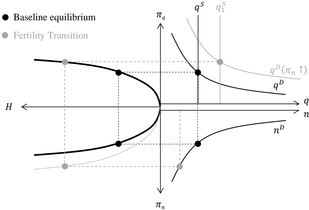
Figure 4 Comparative Static Analysis during the Fertility Transition
