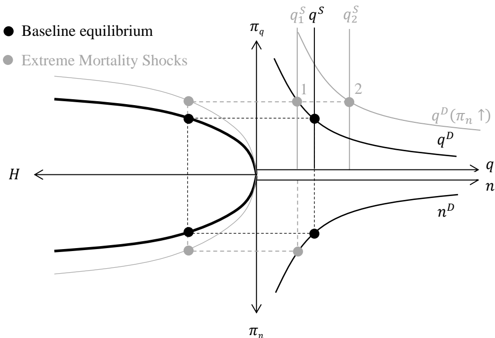
Figure 2 Comparative Static Analysis during the Black Death
