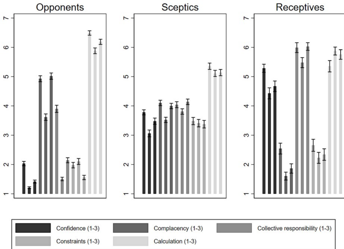
Fig. A1. Detailed Class Characteristics: 5C Scale (All 15 Items). Notes: Results refer to mean values of the 5C scale for vaccination attitudes, separately for each class as identified by the LCA. The mean values shown here are those of the initial 5C scale, measured on a 7-point Likert scale. See Tables A3-A5 for the condensed scale. In order to better illustrate class differences regarding the 5C vaccination hesitancy scale, the graph employs definite class assignment where respondents were assigned to the class with the maximum predicted probability.
