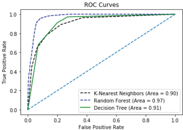
Figure 4. ROC Curves for Classification Algorithms
