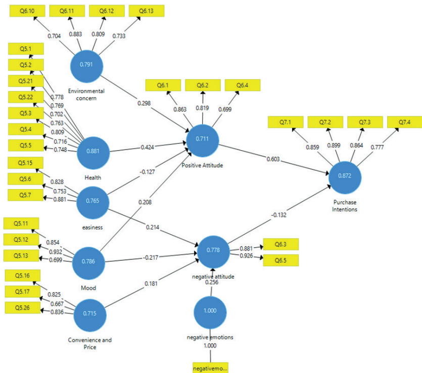
Figure 2. Research Model
