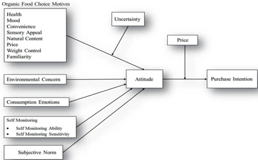
Figure 1. Research Model
