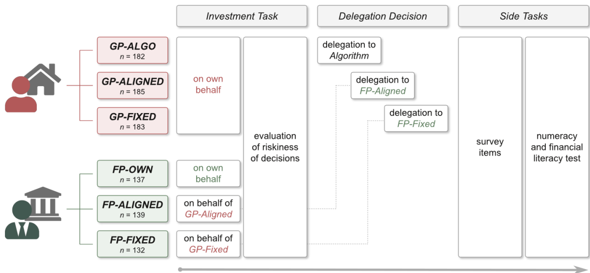
Figure 1: Flow chart of the experiment. This figure illustrates the sequence of tasks for participants in our experiment. First, participants were randomly assigned to one treatment and completed 25 investment decisions. Then, participants from the general population could delegate their investment decision to an agent in a delegation decision stage. Finally, all participants completed several side tasks, including self-reported items on economic preferences and supplementary survey questions, a financial literacy test, and a numeracy inventory.
