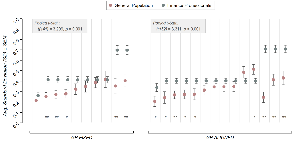
Figure H1: Portfolio risk of clients asking the agent to take more risk when delegating. This figure shows the average portfolio risk across the 25 investment decisions ( SD ; normalized to 1) of those clients that choose to delegate and ask the agent to take more risk than they believe they took in their own decisions, separated for the treatments GP-FIXED and GP-ALIGNED (red dots). The blue dots indicate the mean portfolio risk across the 25 investment decisions ( SD ) of agents that serve as potential matching partners, i.e., those in the corresponding treatment deciding for clients with the risk level that matches their desired risk level when delegating. Error bars indicate standard errors of the mean ( SEM ) and are clustered on the individual level for agents. Asterisks indicate significant differences on the principal-agent level and are based on two-sample t -tests (with clustered standard errors); * p < 0.05 , ** p < 0.005 . Aggregate comparisons between clients' and agents' portfolio risk per treatment are reported in the gray boxes. t -statistics are based on ordinary least squares regressions of portfolio risk on an indicator variable for "agent," controlling for risk profile indicators, with standard errors being clustered on the individual level.
