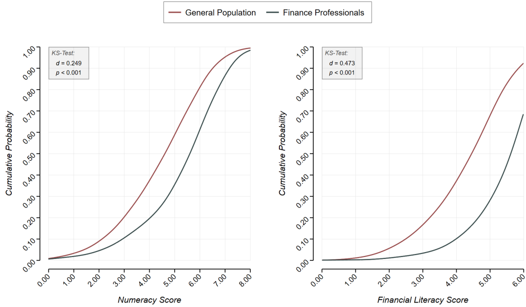
Figure 2: Numeracy and financial literacy scores. This figure shows empirical cumulative density distributions (based on Gaussian kernels with a bandwidth of 1) for participants’ numeracy and financial literacy scores, respectively. Kolmogorov-Smirnov-tests are reported in the light gray boxes ( n = 958 ).
