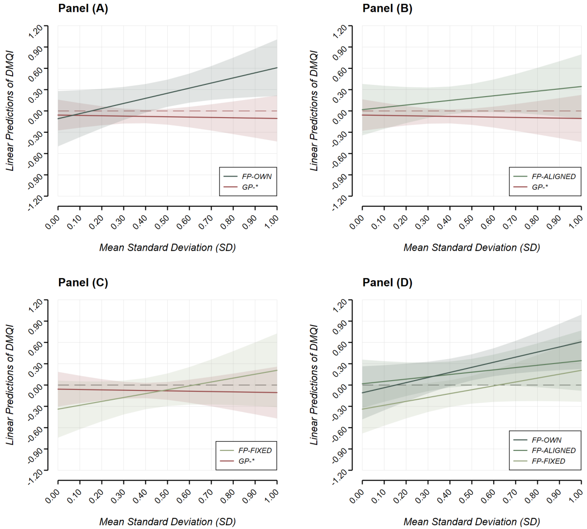
Figure 4: Decision-making quality (DMQI) conditional on portfolio risk. This table shows linear predictions of the decision-making quality index (DMQI) conditional on the mean standard deviation (SD; normalized to 1) across the 25 items in the allocation decision task (normalized to 1) after ordinary least squares regressions with robust standard errors (see Tables 3 and 4. Panels (A)–(C) ). Predictions of DMQI separated for the general population sample (pooled across treatments) and finance professionals deciding on their own behalf (FP-OWN), finance professionals deciding on behalf of clients receiving a flat payment (FP-FIXED), and finance professionals deciding on behalf of clients facing aligned incentives (FP-ALIGNED), respectively. Panel (D) Predictions of finance professionals’ DMQI separated for the three treatments FP-FIXED, FP-ALIGNED, and FP-OWN.
