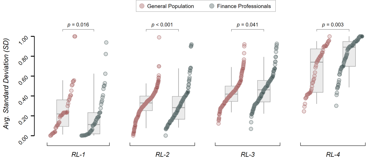
Figure 6: Portfolio risk conditional on self-ascribed risk profiles. This figure shows cumulative distributions and the corresponding boxplots of the mean standard deviation of the 25 allocations in the investment task (normalized to 1), conditional on the perceived riskiness of their choices ( RL-1 ... RL-4 ), separated for the general population sample (pooled across all treatments) and the sample of finance professionals deciding on behalf of clients (i.e., FP-FIXED and FP-ALIGNED ). p -values reported for sample comparisons are based on two-sample Kolmogorov-Smirnov tests. Sample sizes for RL-1 through RL-4 are n_1 = 102 , n_2 = 402 , n_3 = 318 , and n_4 = 136 .
