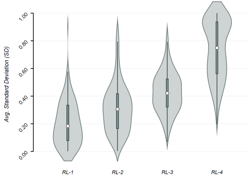
Figure 7: Portfolio risk conditional on clients’ requested risk level. This figure illustrates the distribution (Gaussian kernel) of the average standard deviation of the 25 allocations in the investment task (normalized to 1), conditional on the risk level ( RL-1 ... RL-4 ) indicated by clients for treatments FP-FIXED and FP-ALIGNED . Sample sizes for RL-1 through RL-4 are n_1 = 77 , n_2 = 60 , n_3 = 68 , and n_4 = 66 .
