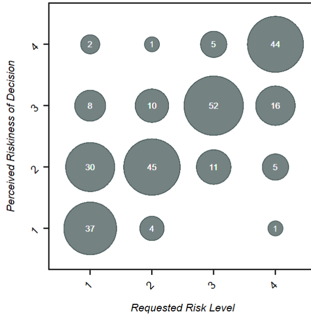
Figure 5: Desired risk conditional on risk perception. Risk level agents are asked to comply with when deciding on behalf of clients vs. agents’ perception of the riskiness of their actual decisions ( n = 271 ).
