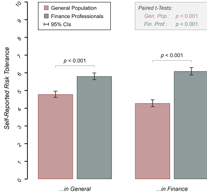
Figure 3: Self-reported risk tolerance. This figure depicts the mean levels of risk tolerance (self-reported on scales from 1 to 10) in general and in financial matters, respectively, separated for the general population sample and the finance professionals sample. p -values reported above the bars indicate comparisons between the subject pools and are based on two-sample t -tests ( n = 958 ). p -values reported in the box are based on paired-sample t -tests with sample sizes of 550 (general population) and 408 (finance professionals), respectively.
