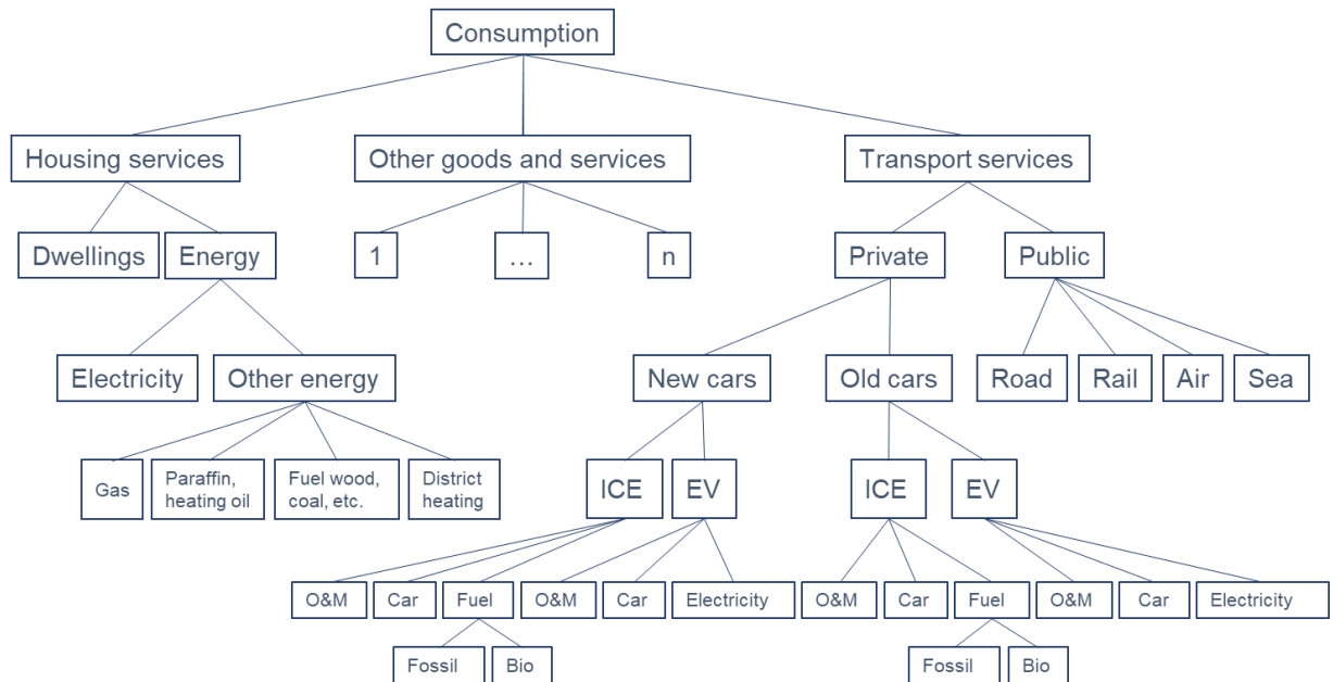
Figure 3.1 The CES function of private material consumption in SNOW
