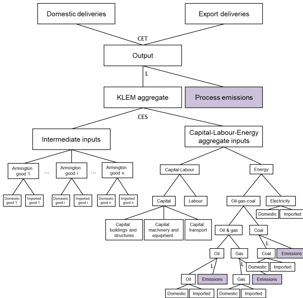
Figure 3.2 Nested CES production function in SNOW, with emissions highlighted
