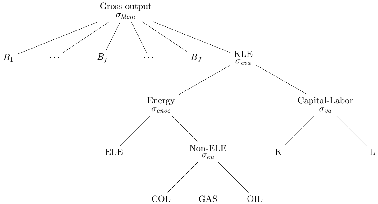
Figure 8. Production structure for final goods non-energy sectors g \in G = \{AGR, EIS, TRN, SRV, MAN\} and refining of crude oil c \in C = \{OIL\} .
