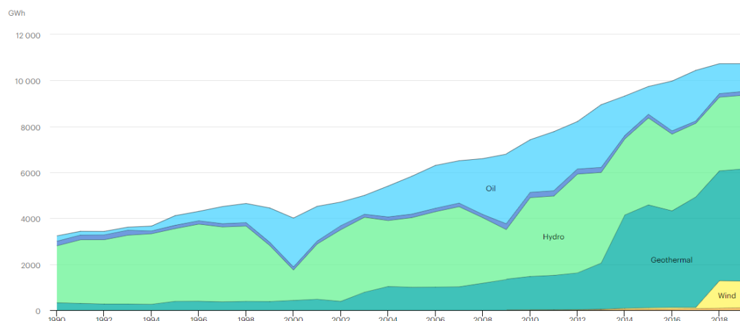
Figure 3. Kenya electricity generation by source 18
