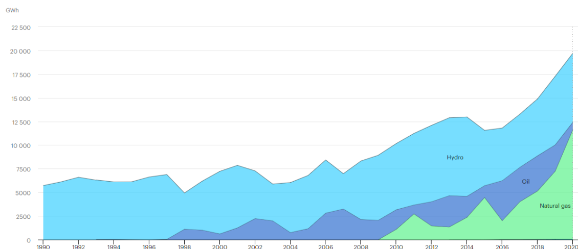
Figure 2. Ghana electricity generation by source 16
