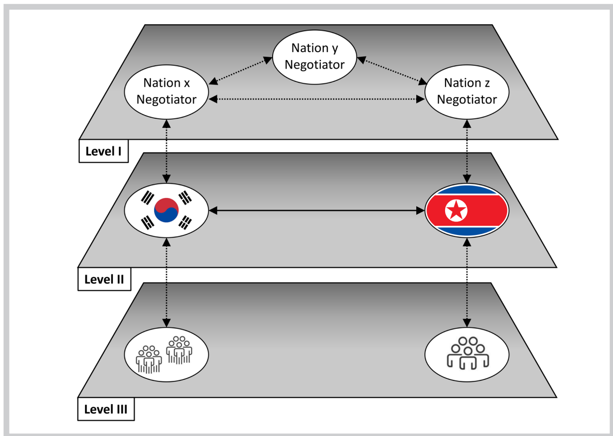
Figure 1: Three-Level Game 2
