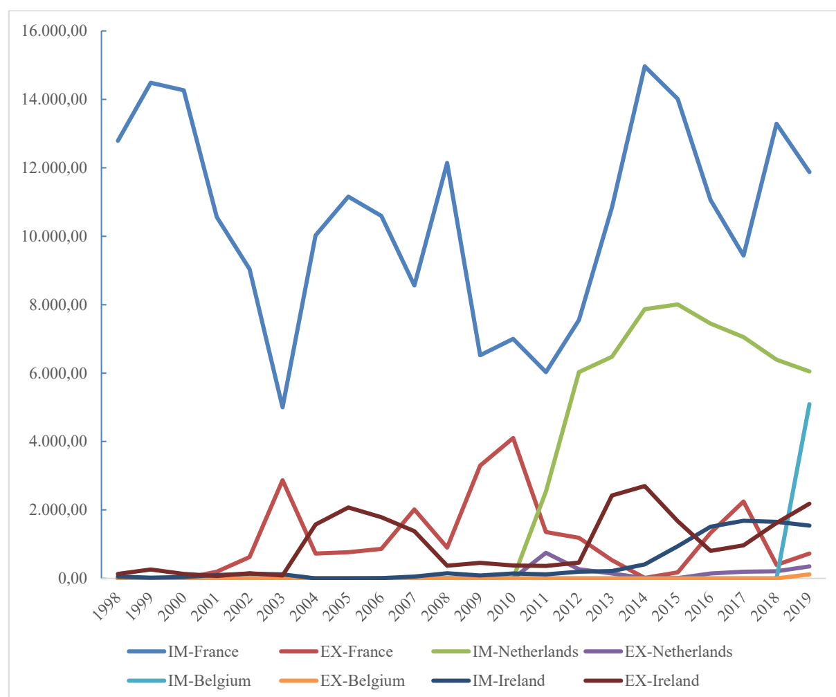
Figure 4 UK Imports and Exports of Electricity (1998-2019)
