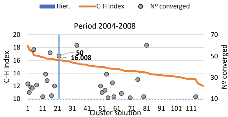
Figure A2.7 Robustness check with k-means random centroids
