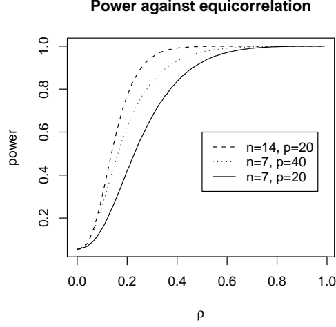
Figure 1: Empirical rejection probabilities of \phi_{np} for the case of equicorrelation
