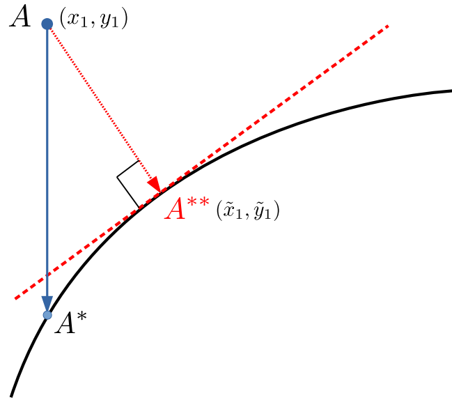
Figure 4: Fragment of the Environmental Kuznets frontier and the exact solution to find h
