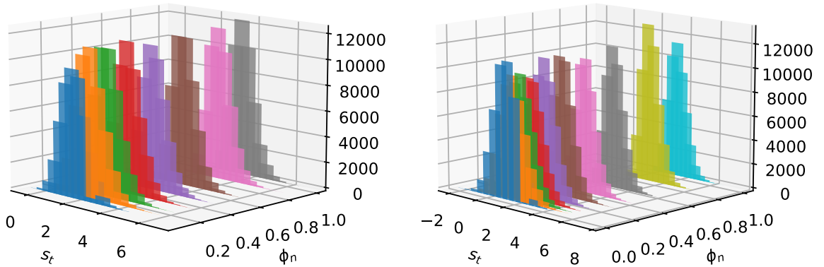
Figure 2: Tempering of the state distributions of \ln(\sigma_{t,i}^2) in 1978 (Q2)
