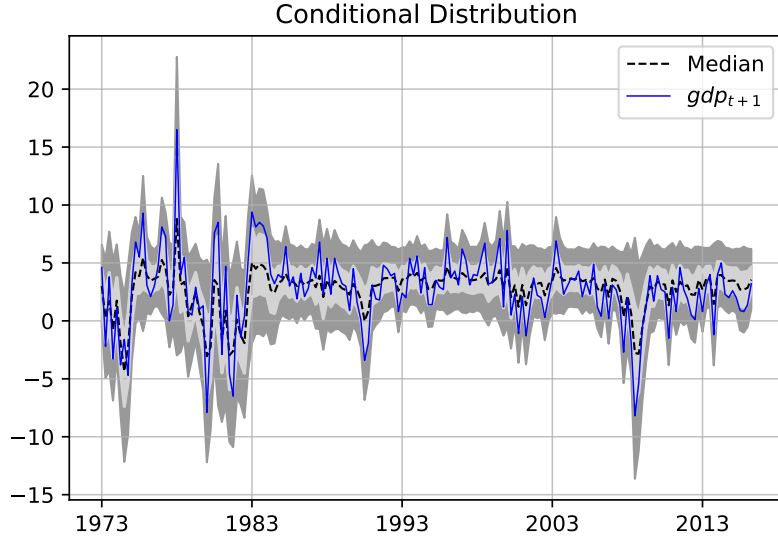
Figure 7: The one-step ahead forecasting distribution for one-quarter ahead GDP growth
