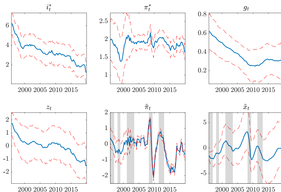
Figure 10: Euro area latent macro variables
