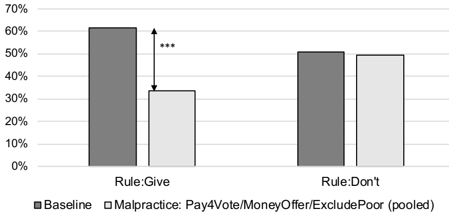
Figure 3: Effect of interventions Pay4Vote , MoneyOffer and ExcludePoor (pooled) on the power of elected rules to change behavior. Bars show decrease (in %) in the share of subjects choosing to not give (give) after the election of Rule:Give ( Rule:Don't ) relative to the share of subjects choosing to not give (give) in the absence of a rule. The graph is based on type-weighted averages, stars denote significance of population average treatment effect of Malpractice (Pooled) on compliance with Rule:Give , *** p < .01 , see Table 3.
