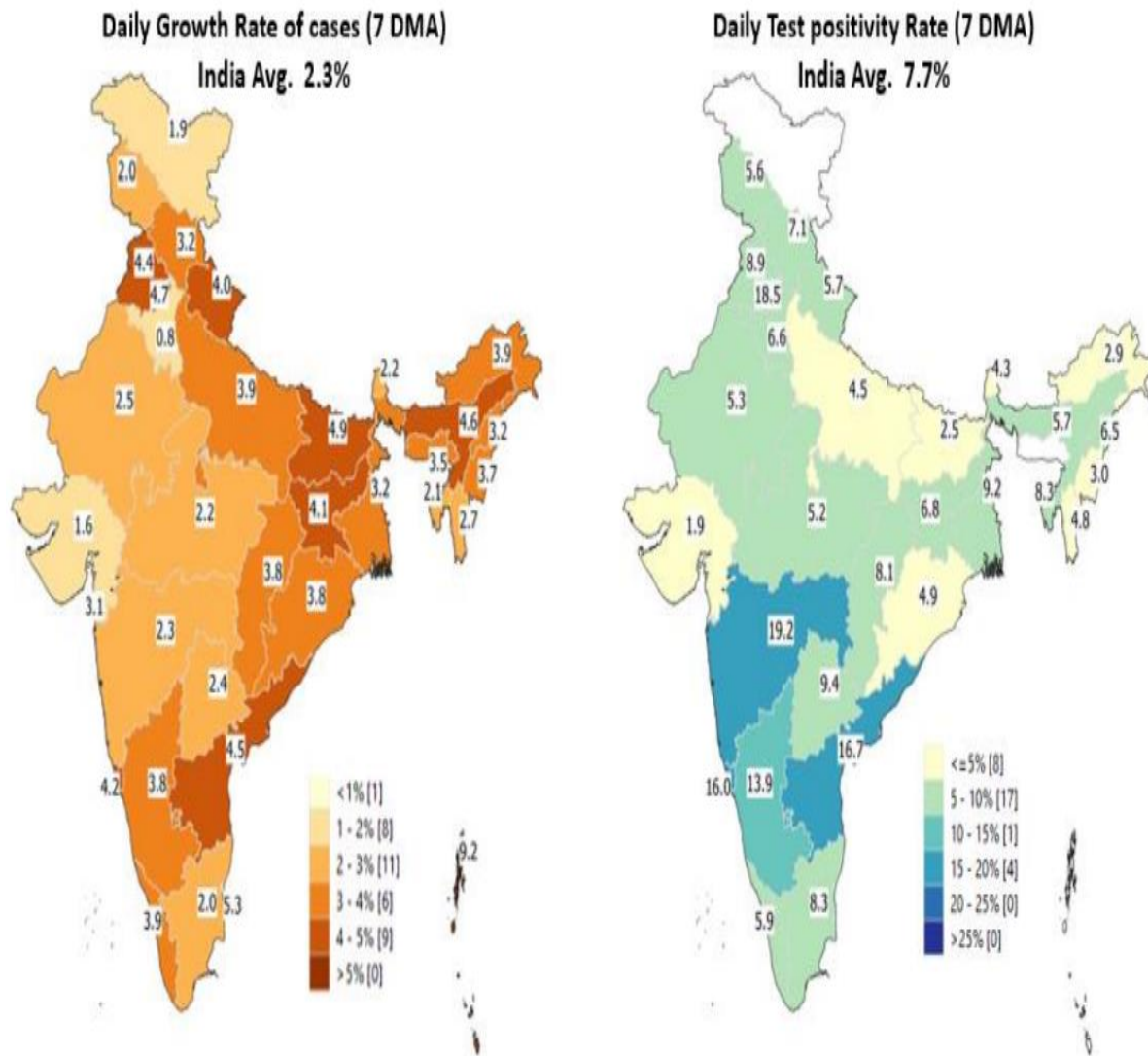
Figure 5: Daily growth rate of COVID-19 cases and Daily Test Positivity rate in various states in India
