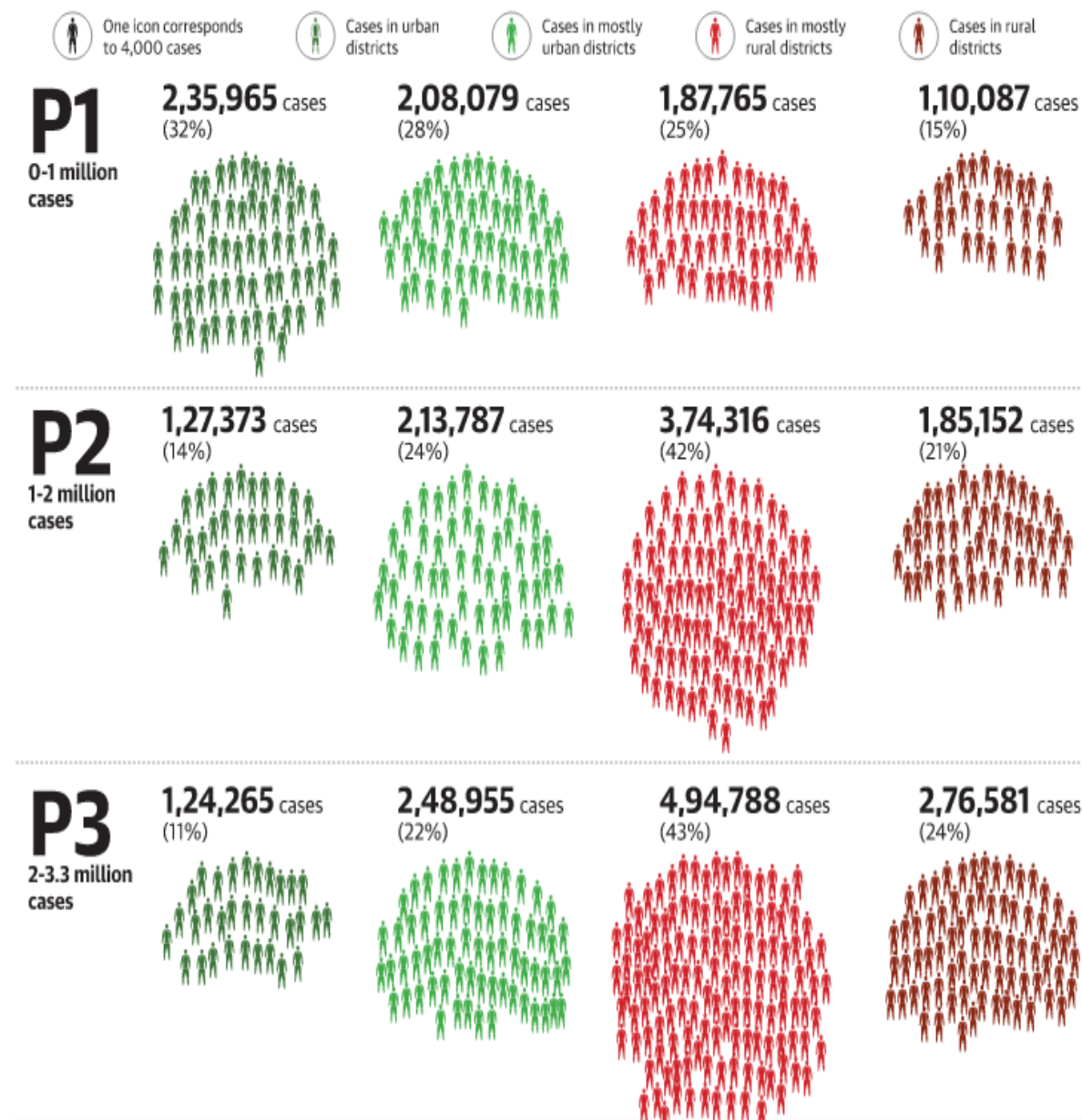
Figure 11: The total number and % share of India’s new cases recorded during three stages: P1 (cases between 0 and 1 million), P2( cases between 1 million and 2 million) and P3 (cases between 2 million and 3.3 million cases) across urban, mostly urban, mostly rural and rural districts
