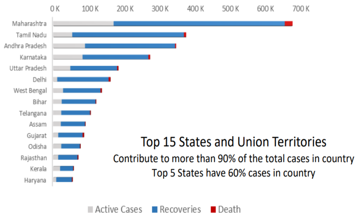
Figure 2: Top 15 States and Union Territories contributing to 90% COVID-19 cases in India.
