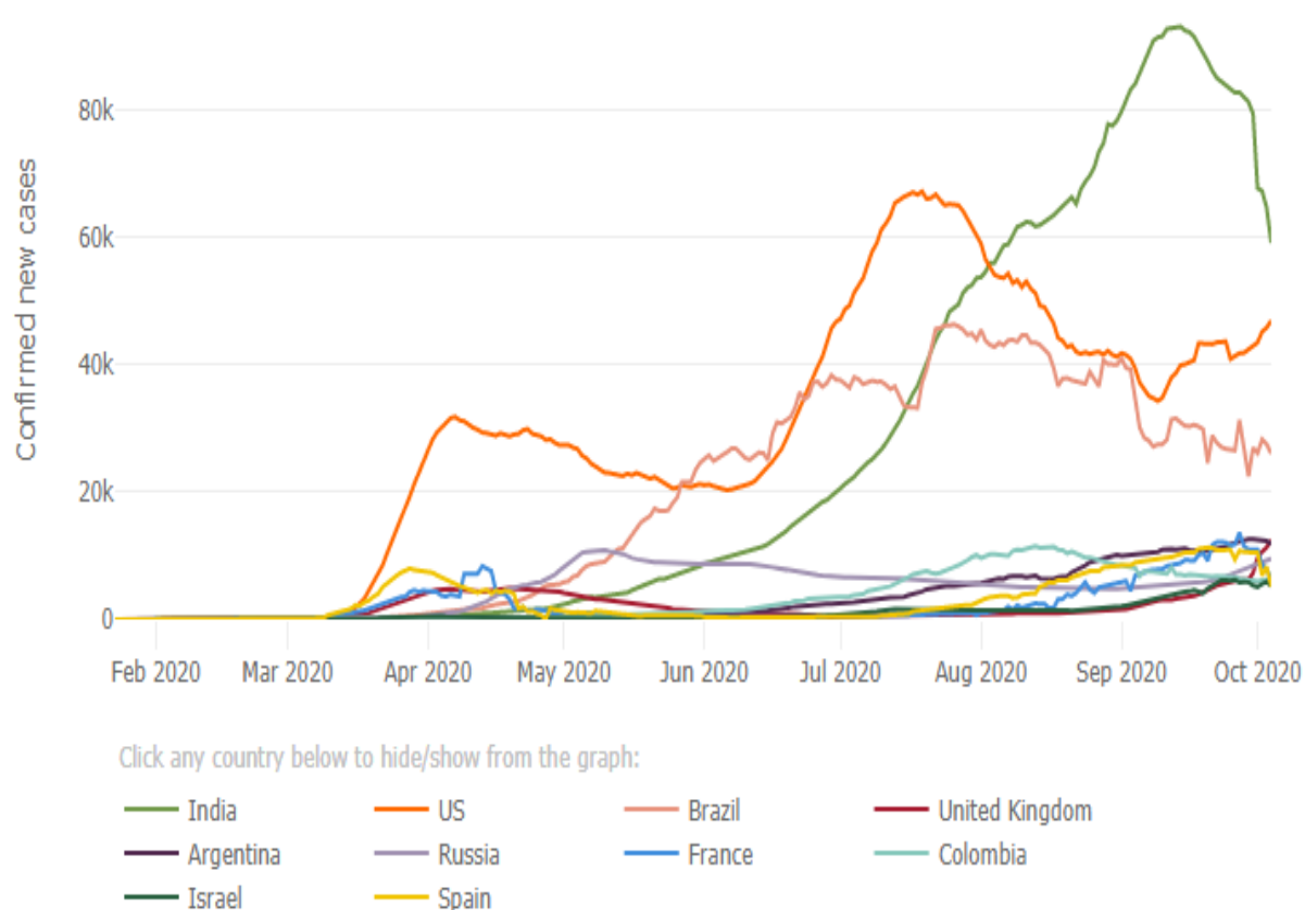
Figure 1: Daily confirmed new cases (7-day moving average) from Feb 2020 to October 2020 in India and other countries
