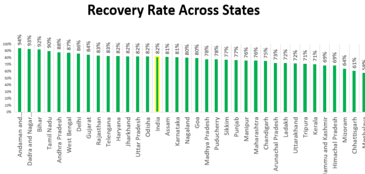
Figure 8: Recovered cases across states in India
