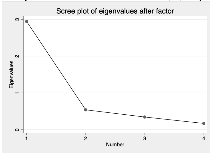
Figure A1: Scree Plot of Confirmatory Factor Analysis Hypothesizing That All Four Identity Variables Load onto One Distinct Factor (i.e., occupational identity).
