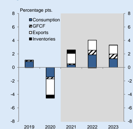
Figure 9.2: Import adjusted expenditure-side contributions to GDP growth
