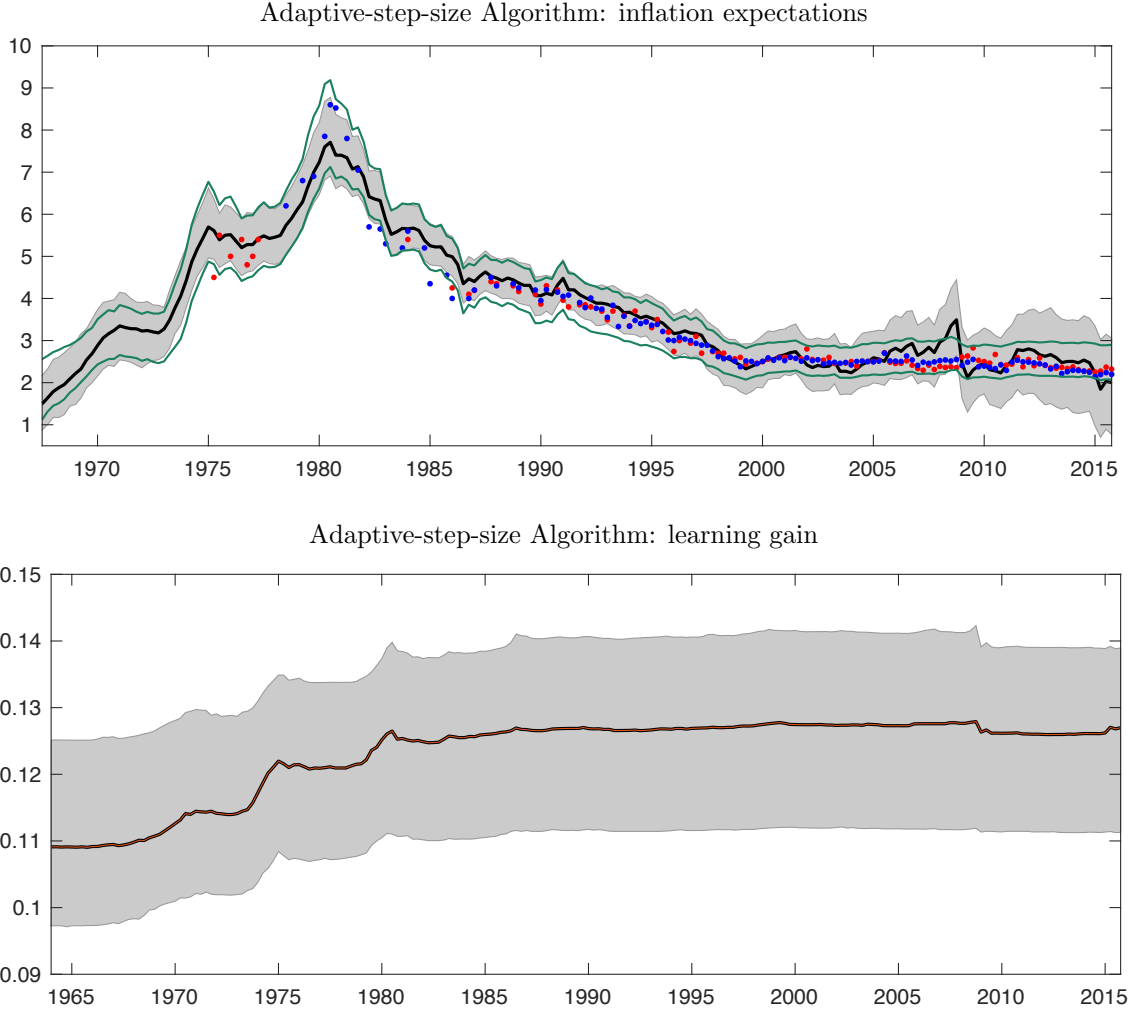
Figure 8: Adaptive-step-size-algorithm.
