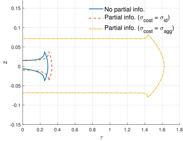
Figure 7: Optimal policies implied by the estimated models
