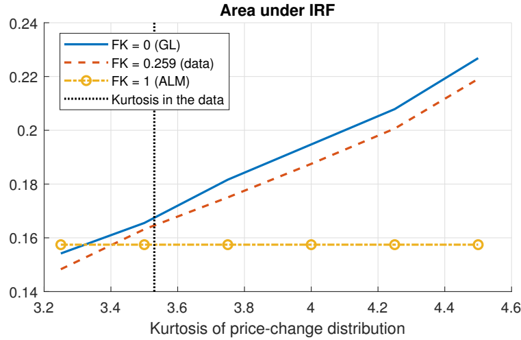
Figure 16: Area under impulse response functions as a function of the kurtosis of price-change distribution.
