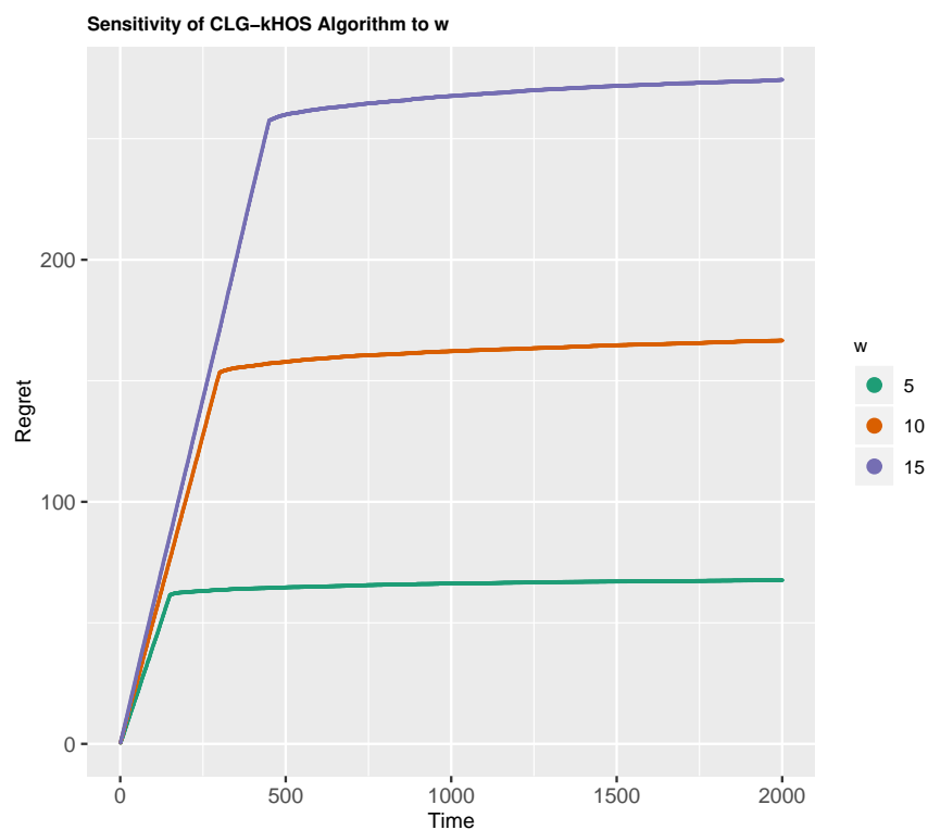
Figure 1: Comparison of Cumulative Regrets of the CLG-κHOS algorithm for values of w \in \{5, 10, 15\} , s_t \equiv s = 0.5 and \kappa_t \equiv \kappa = w/2 .
