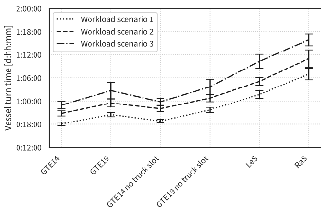
Figure 3: Vessel turn time
