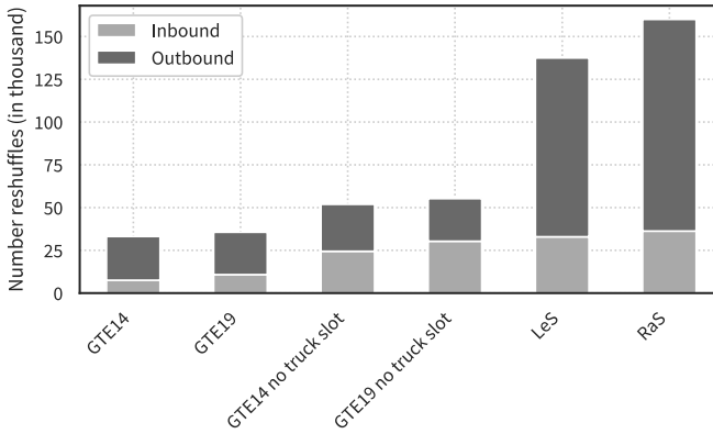
Figure 5: Number of reshuffles over the simulation period
