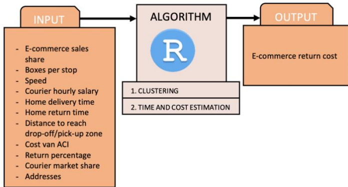
Figure 1: Model architecture
