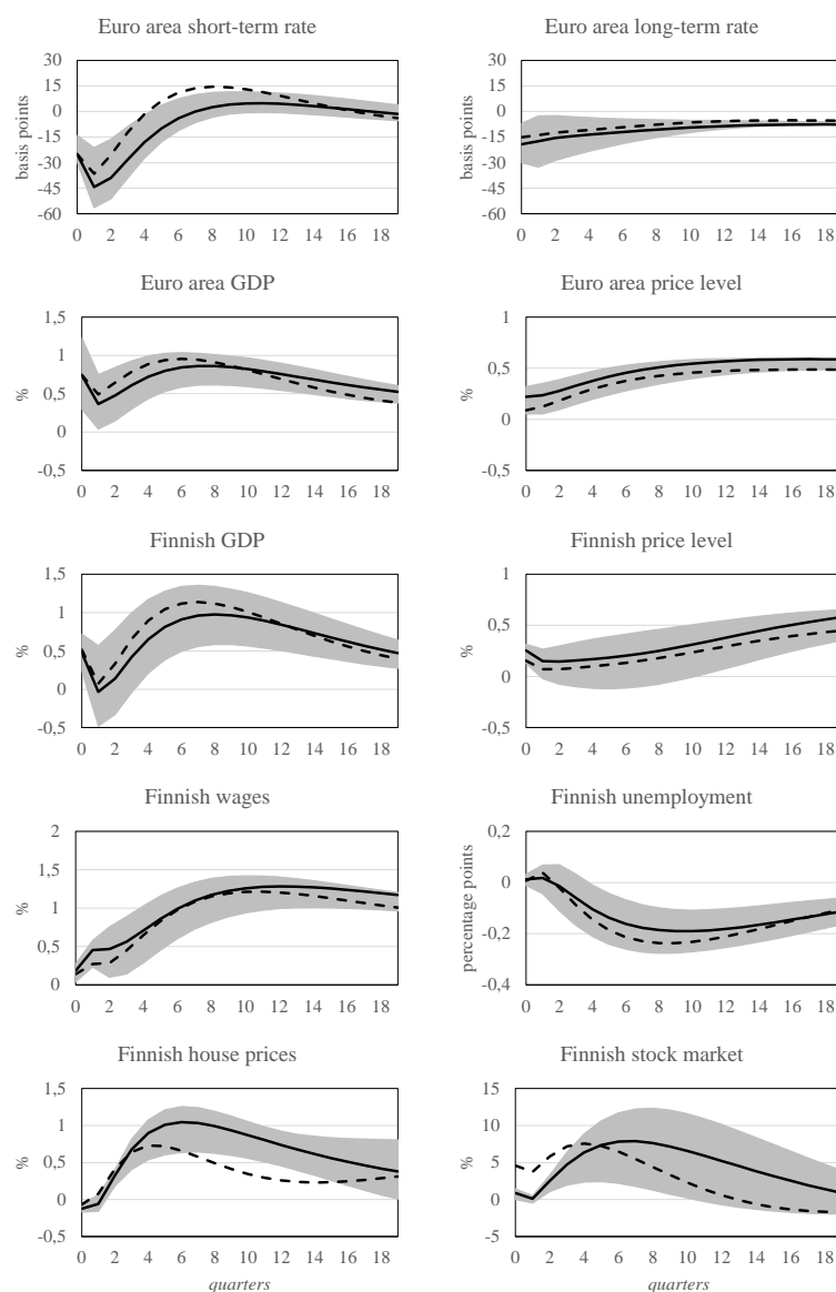
Figure C.1. Aggregate impulse responses to a 25 basis point expansionary conventional monetary policy (MP) shock. Note: Solid black lines denote period-wise median impulse responses, and grey areas denote 68% period-wise bands of the identified set in the baseline SVAR specification. Dashed black lines show period-wise median impulse responses computed from the alternative specification with the DAX index.
