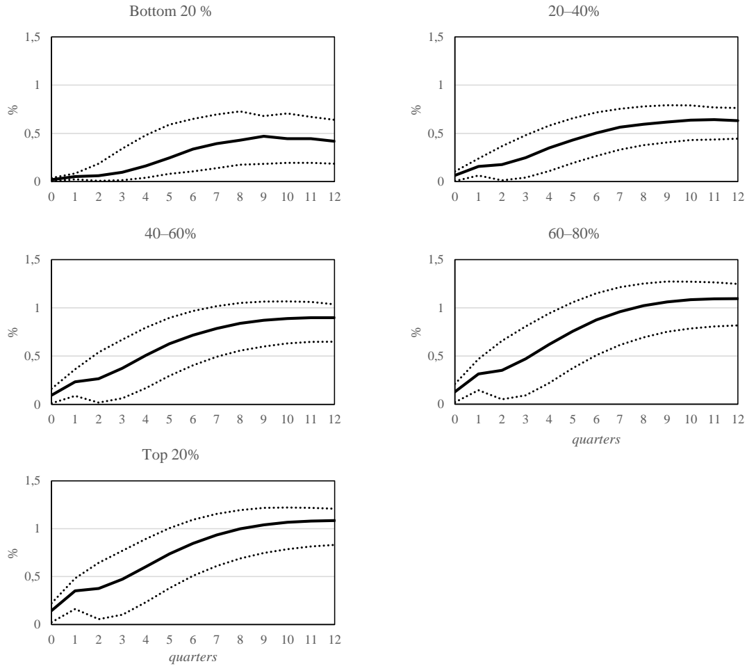
Figure 10. Response of households' mean gross income to an expansionary conventional monetary policy (MP) shock of 25bp, in percent deviations from initial level, by gross income quintiles. Note: The solid lines show the average responses in each quintile that correspond to the period-wise median aggregate impulse responses, and the dotted lines correspond to the 68% period-wise bands of the identified set of the aggregate impulse responses.
