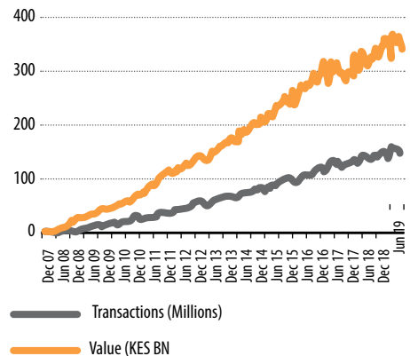
Figure 2: Mobile Payments
