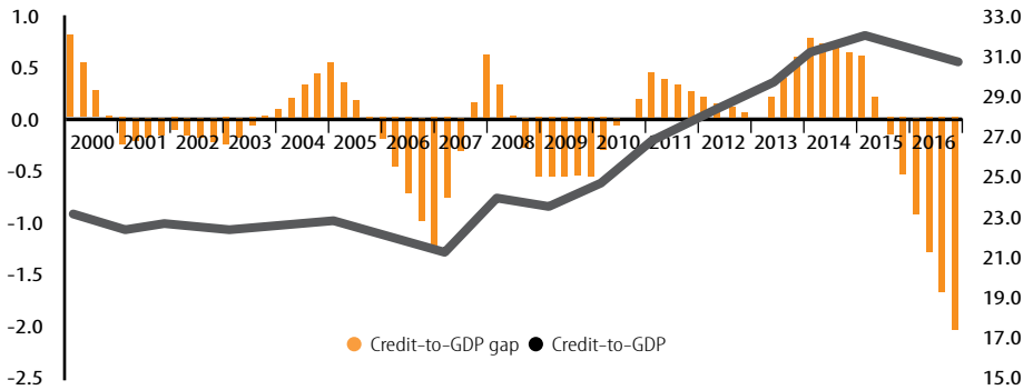
Figure 2: Credit-to GDP Gap (Left Axis) and Credit-to-GDP (Right Axis)
