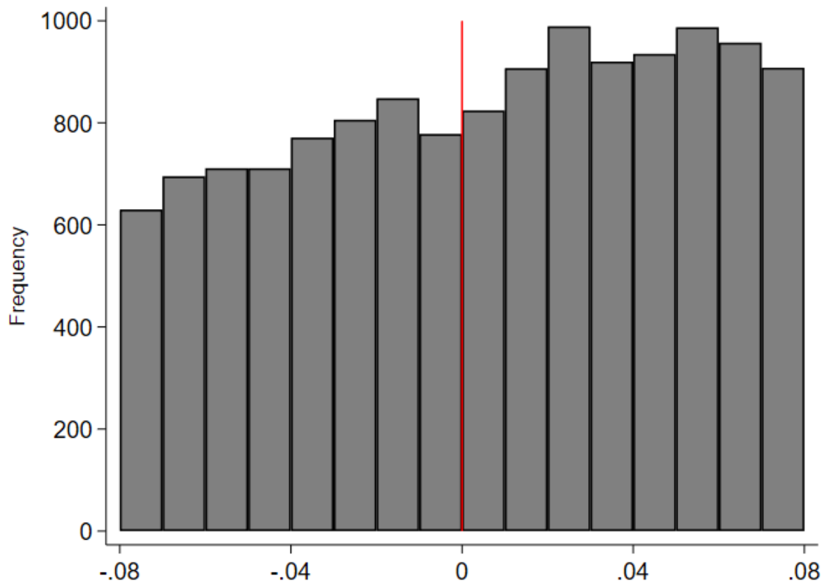
FIGURE E.5 DENSITY OF THE ALIGNMENT RUNNING VARIABLE AROUND THE THRESHOLD
