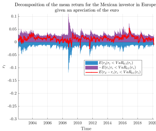
(c) Mexican investment in European equity ( r_d - r_e ) under a EUR appreciation shocks ( r_e )
