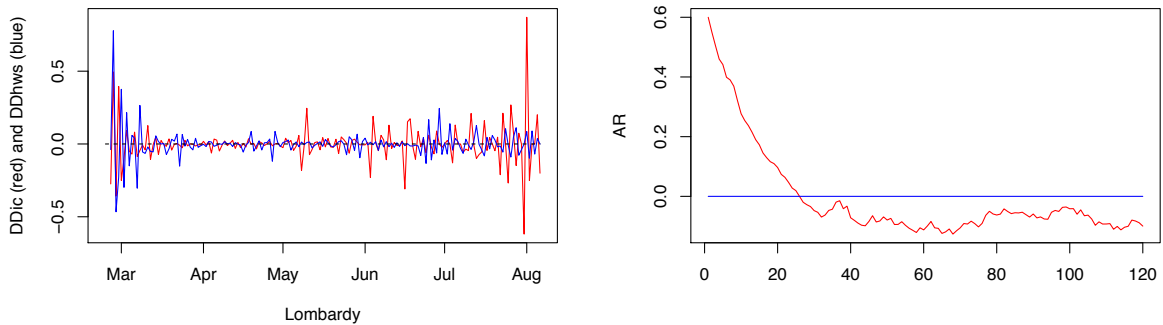
Figure 4: Left: data for \Delta^2 ic = \Delta^2 \log(IC) and \Delta^2 hws = \Delta^2 \log(HwS) for Lombardy, February 24 - August 6, 2020. Red: ic . Blue: hws . Right: simulation of a univariate AR process with mean c , w_t - c = \rho(w_{t-1} - c) + \varepsilon_t with \rho = 0.94 , c = -0.1 , w_0 = 0.6 , \varepsilon_t i.i.d. N(0, \sigma^2) with \sigma = 0.01 .
