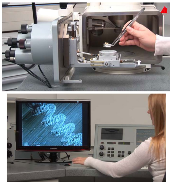
Fig. 3 Operation of an SPM ( https://www.youtube.com/watch?v=GY9lfo-tVfE )
