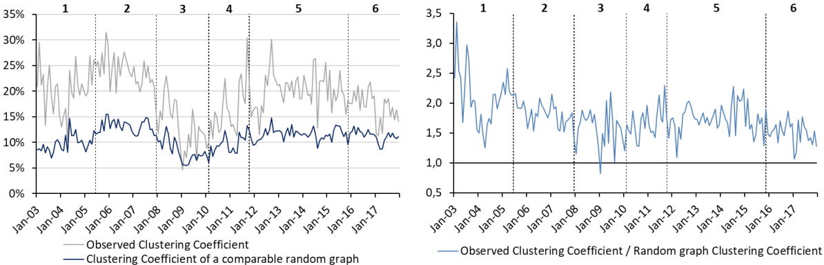
Figure 12 | Clustering coefficient
