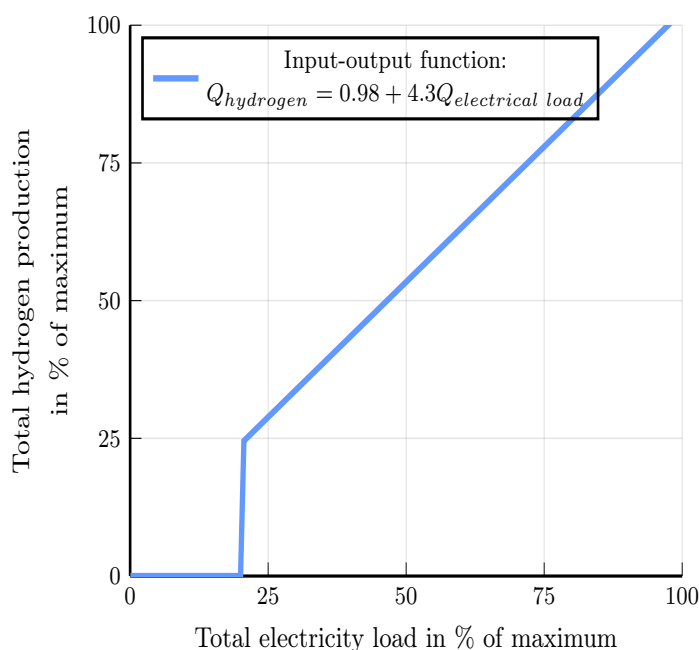
Figure 2: Electrolyser input-output-function (own assumption based on Kopp et al. (2017)).
