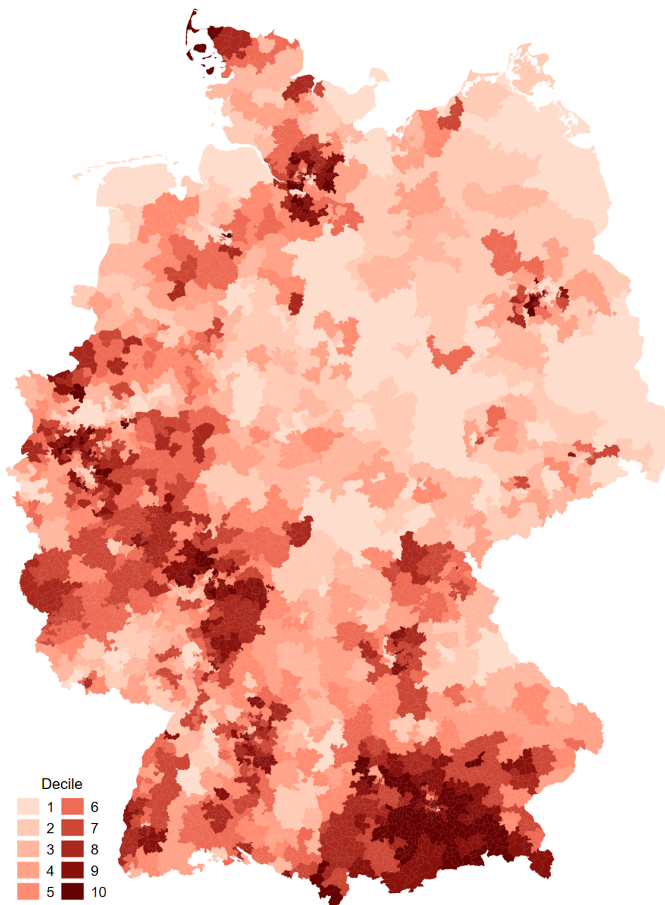
Figure 2: Share of target persons in each PSU (Deciles). Note: We refrain from providing the boundaries of primary sampling units (PSUs). Thus connecting PSUs with same color cannot be distinguished.
