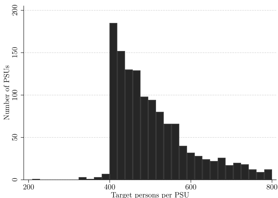
Figure 1: Distribution of the number of target persons per PSU
